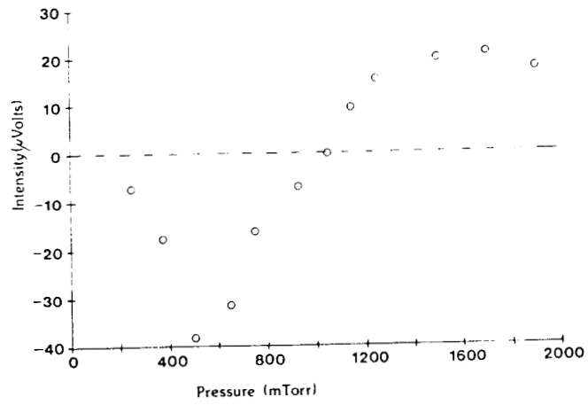
Figure 3: Variation of intensity of LOGE signal for CO 2 as a function of pressure.
