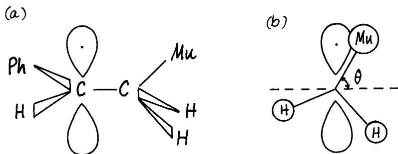
Figure 4. Structure of the phenyl-ethyl radical (a) indicating the singly occupied p_z orbital, perpendicular to the plane of the PhHC moiety. The (muonated) methyl group has some rotational freedom about the C-C bond (viewed along this bond in (b)) but adopts a preferred orientation, \theta = 90^\circ .
