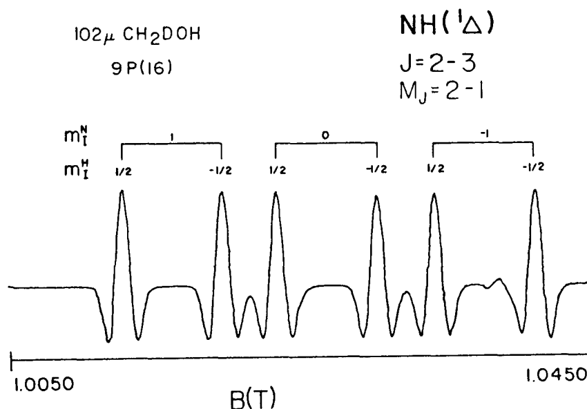
Fig. 1. The J = 2 \leftarrow 3 , M_J = 2 \leftarrow 1 transition of \text{NH}(a^1\Delta) .
