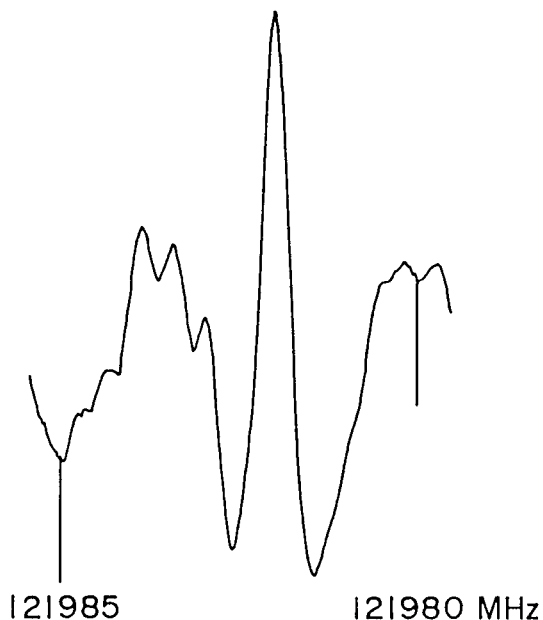
Fig. 1. The J = 11 - 10 transition of ^{18}\text{O}^{13}\text{C}^{34}\text{S} in natural abundance (0.96 ppm) observed by an integration of 50 s with the 3.5 m free space cell and source modulation.
