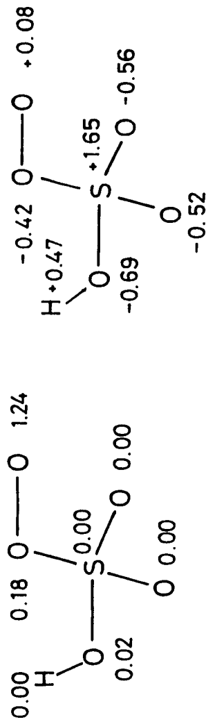
Figure 5. Atomic spin densities and net atomic charges of the HOS(O) 2 O 2 radical
