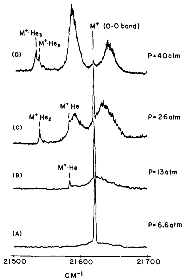
Fig. 5. Laser Excitation Spectra of C_6F_6^+ ( = M^+ ) Expanded in Pure He. The relevant stagnation pressure ( P ) is indicated on each trace.
