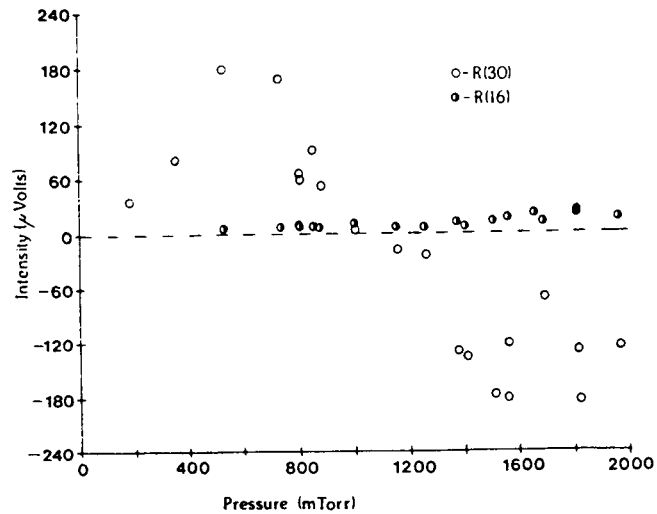
Figure 6: Variation in intensity of R(30) and R(16) over the pressure range 200 to 2000 mTorr \text{NH}_3 .
