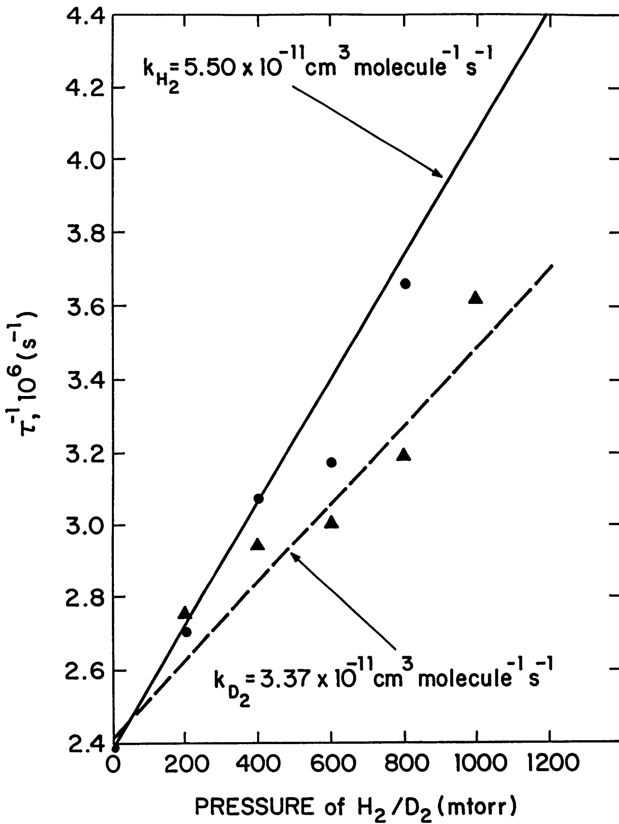
Fig. 3. Quenching plot of the inverse of the fluorescent lifetime, \tau^{-1} , versus pressure of H 2 or D 2 .
