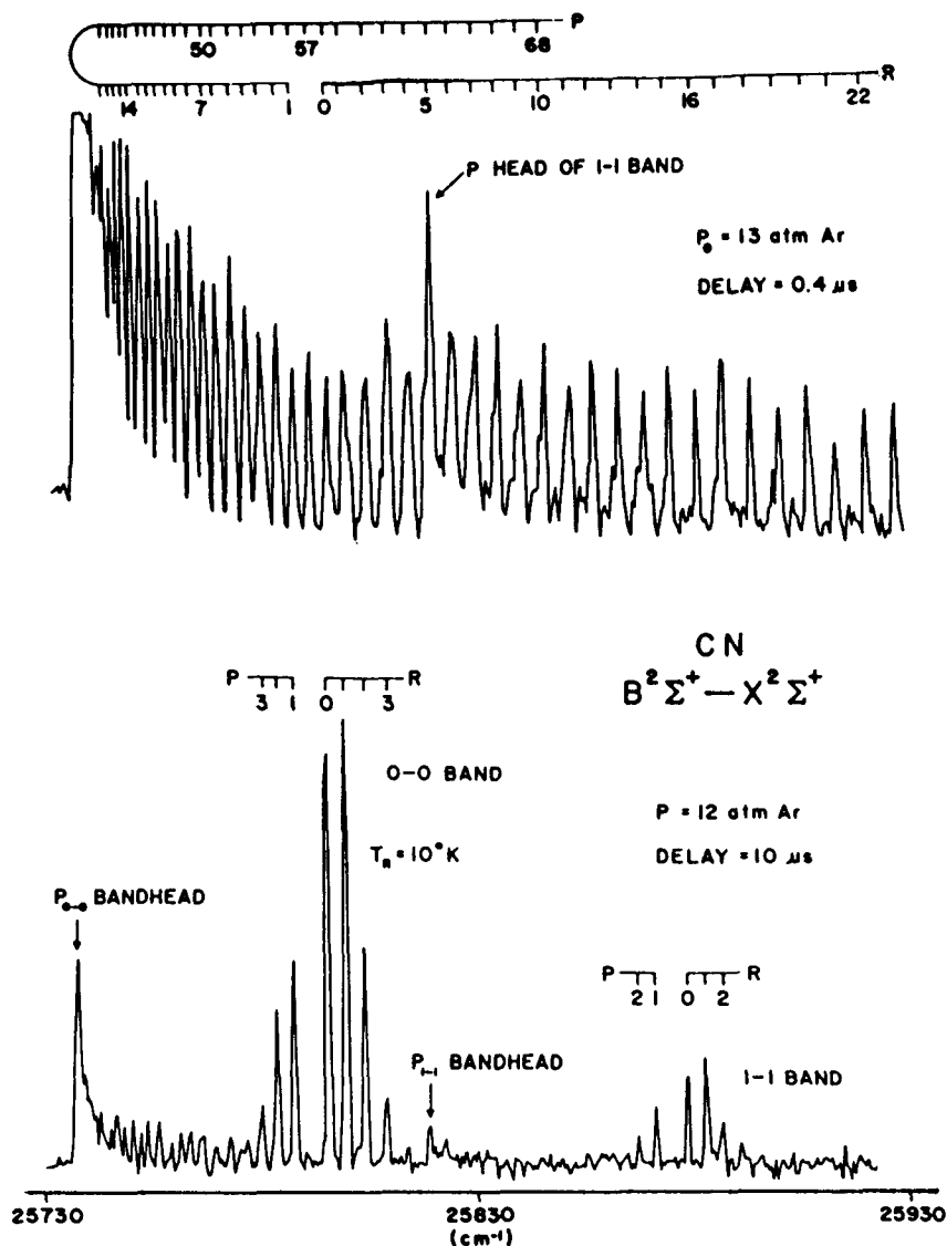
Fig. 6. Laser-induced fluorescence spectra of the CN free radical produced by the ArF laser photolysis of BrCN in an Ar free jet expansion. In the upper trace, the probe and photolysis laser are nearly overlapped in space and time, and the CN distribution detected is nascent or near nascent. In the lower trace, the probe laser has been displaced downstream by 10 \mu\text{sec} in time and 6 mm in distance. Large redistributions in rotational populations are clear. The rotational assignments for the R and P branches are as indicated.
