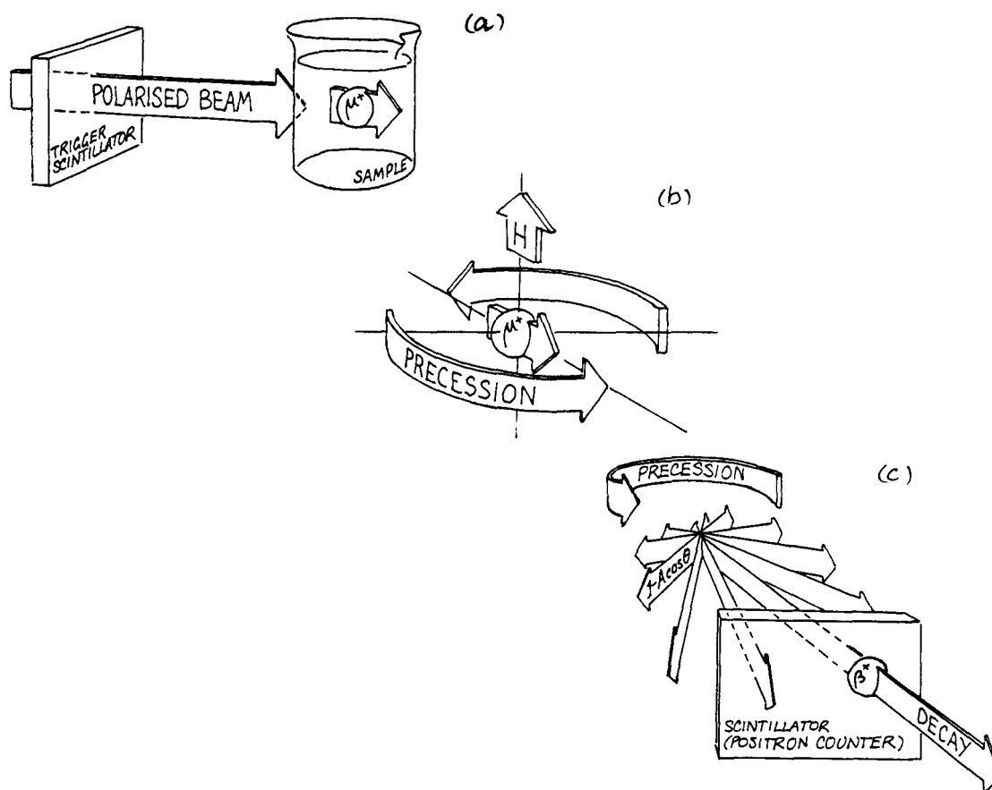
Figure 1. The \mu\text{SR} method. Implantation (a), Larmor precession (b) and radioactive decay (with detection of the emitted positron) (c) of spin-polarised muons. The polar diagram for the probability of positron emission rotates with the muon polarisation (just as that for \gamma -ray emission does in Perturbed Angular Correlation experiments).
