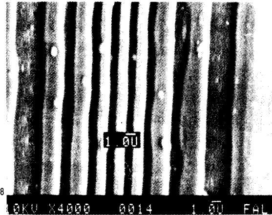
FIG. 2. Submicrometer-resolution etching of poly-Si surface by ArF laser photolysis of COF 2 .
