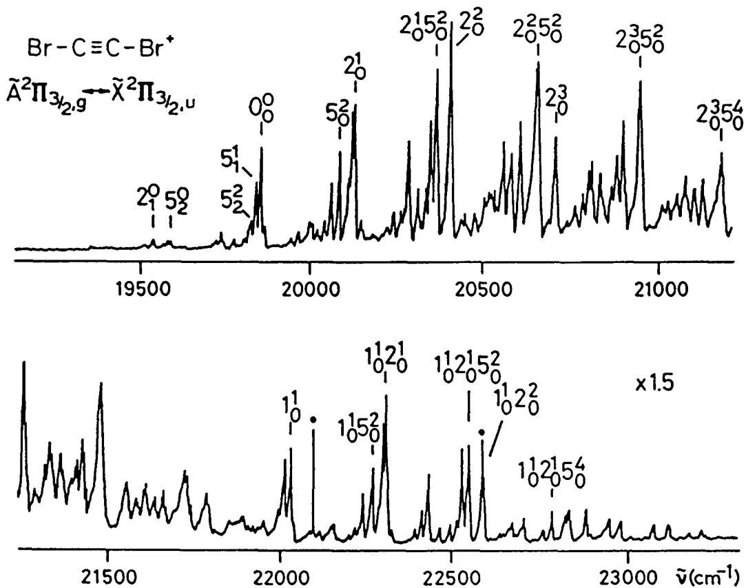
FIG. 5. Part of the laser excitation spectrum of the \tilde{A}^2\Pi_{3/2,g} \leftarrow \tilde{X}^2\Pi_{3/2,u} transition of Br-C≡C-Br + in the gas-phase, resolution 0.02 nm. Atomic lines are marked with a dot.
