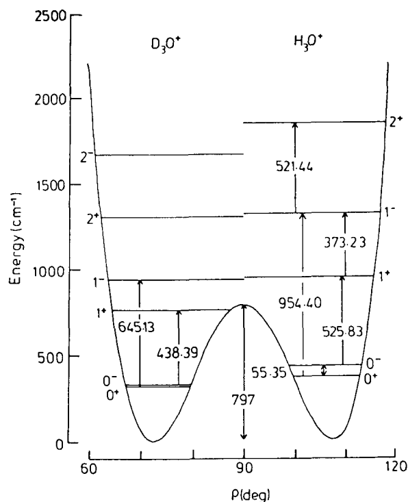
6. The inversion potential of H_3O^+ ( D_3O^+ ) showing the lowest vibrational levels and the transitions so far detected by diode laser spectroscopy.
