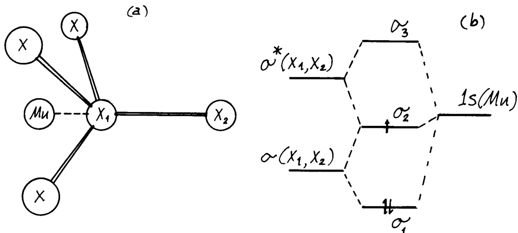
Figure 6. Structure A for the Mu' centre (a), and a qualitative level diagram (b) indicating the interaction of the \sigma and \sigma^* orbitals for the stretched bond X_1-X_2 with muonium. The singly occupied molecular orbital retains some hydrogenic character.
