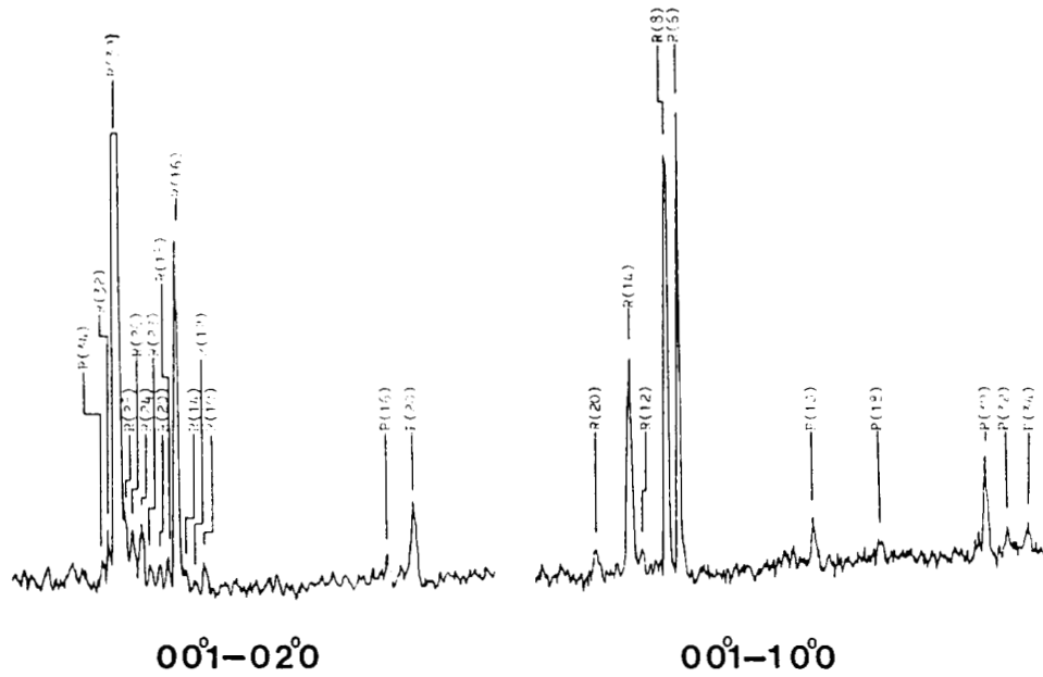
Figure 4: LOGE signal from NH 3 for the 00 0 -02 0 and 00 0 -10 0 bands of the CO 2 laser.
