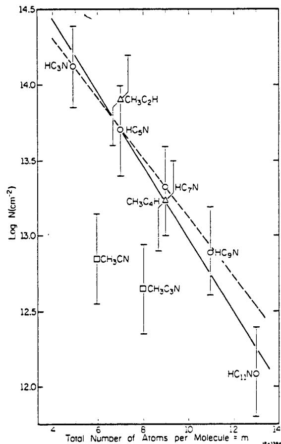
Fig. 6 - The logarithms of the revised column densities (ordinate) plotted against m , the total number of atoms per molecule (abscissa) for the dark dust cloud TMC 1 (from Snyder, Dykstra, and Bernholdt 1985a). Solid line-least squares fit for \text{HC}_3\text{N} through \text{HC}_{11}\text{N} (circles). Dashed line-least squares fit for \text{HC}_3\text{N} through \text{HC}_9\text{N} only. The logarithms of the column densities of the \text{CH}_3\text{CN}-\text{CH}_3\text{C}_3\text{N} (squares) and \text{CH}_3\text{C}_2\text{H}-\text{CH}_3\text{C}_4\text{H} (triangles) families are plotted but not included in the least squares fitting.
