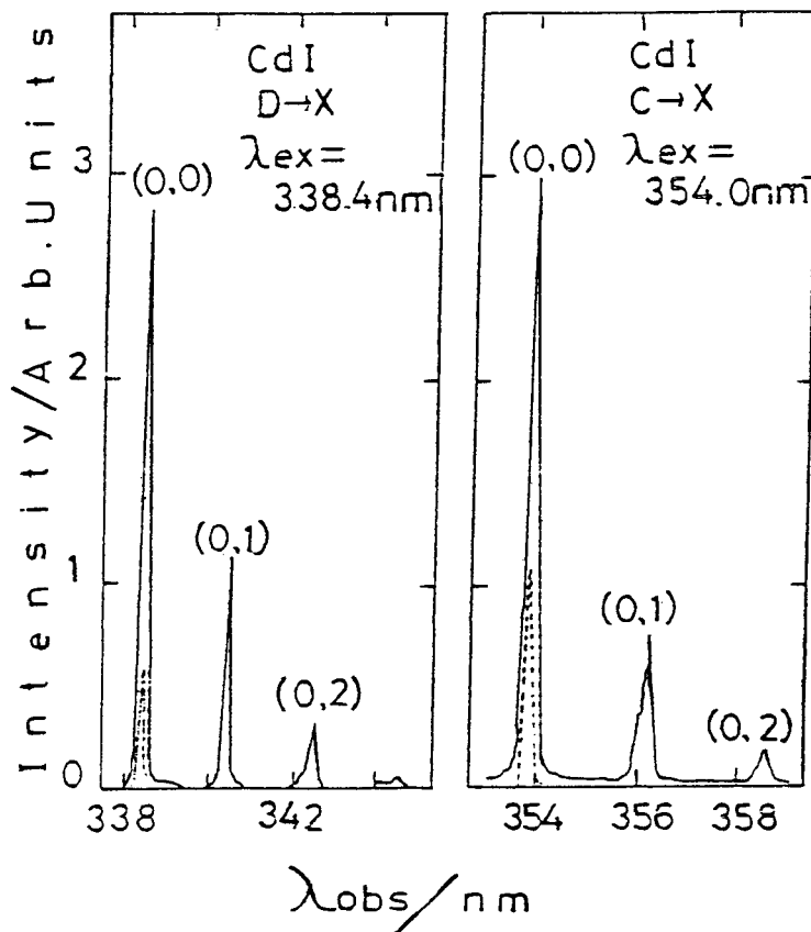
Fig. 2. LIF spectra of CdI radical.
