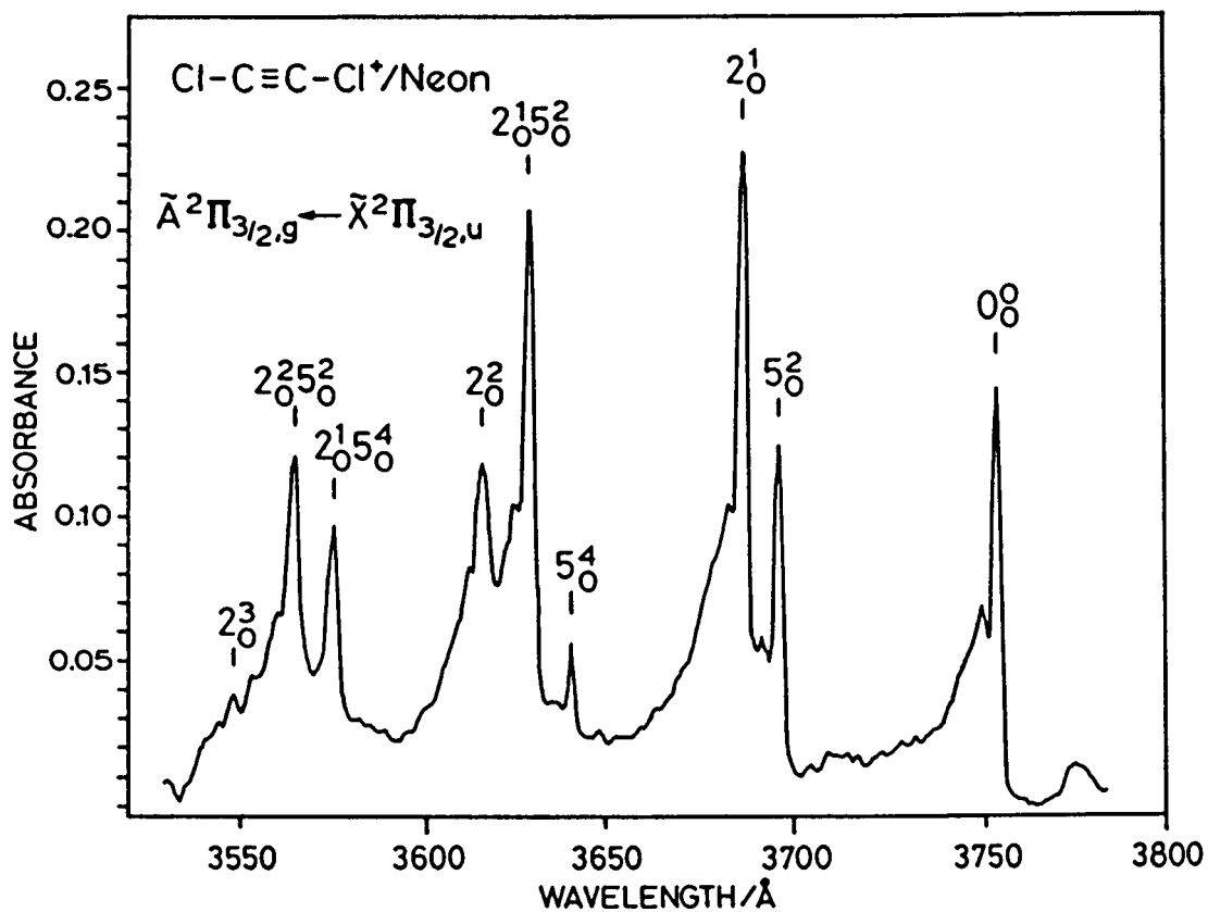
FIG.6. Part of the \tilde{A}^2\Pi_{3/2,g} \leftarrow \tilde{X}^2\Pi_{3/2,u} absorption spectrum of Cl-C≡C-Cl + in a neon matrix, optical resolution 0.1 nm.
