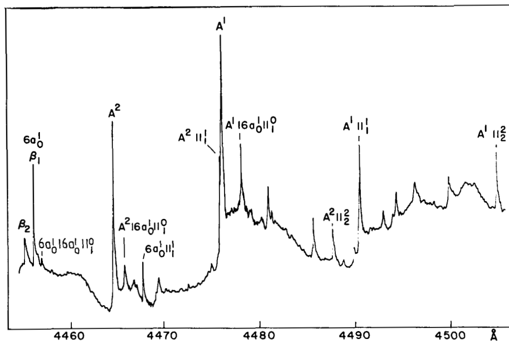
Fig. 1 - Microdensitometer trace of the gas phase absorption spectrum of benzyl between 4450 and 4510 Å.
