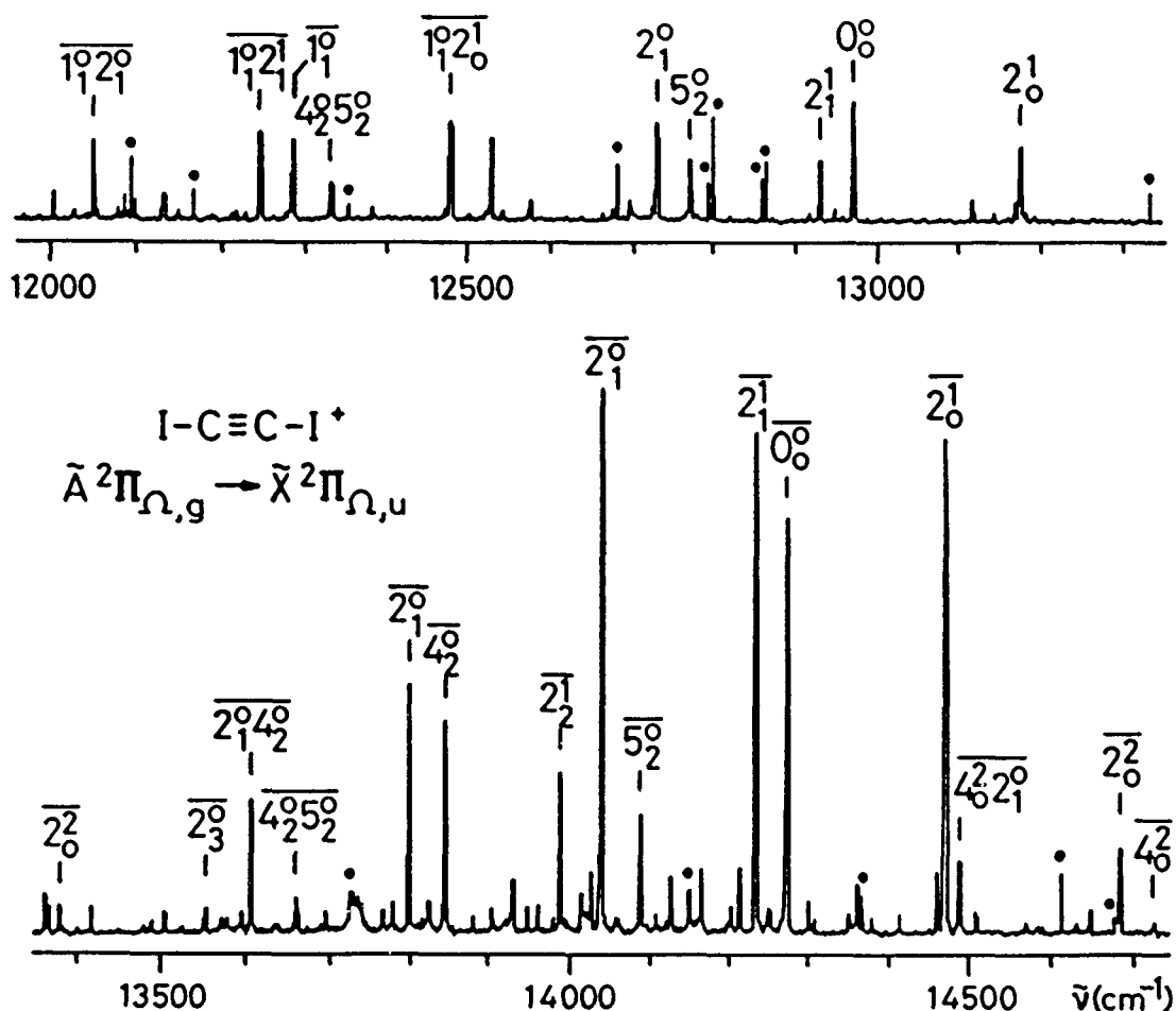
FIG. 4. Part of the \tilde{A}^2\Pi_{\Omega,g} \rightarrow \tilde{X}^2\Pi_{\Omega,u} ( \Omega = 3/2, 1/2 ) gas-phase emission spectrum of \text{I-C}\equiv\text{C-I}^+ in a seeded helium supersonic free jet, resolution 0.03 nm. Some of the vibrational assignments are indicated; a horizontal bar indicates the \Omega = 1/2 system. Helium lines are marked with a dot.
