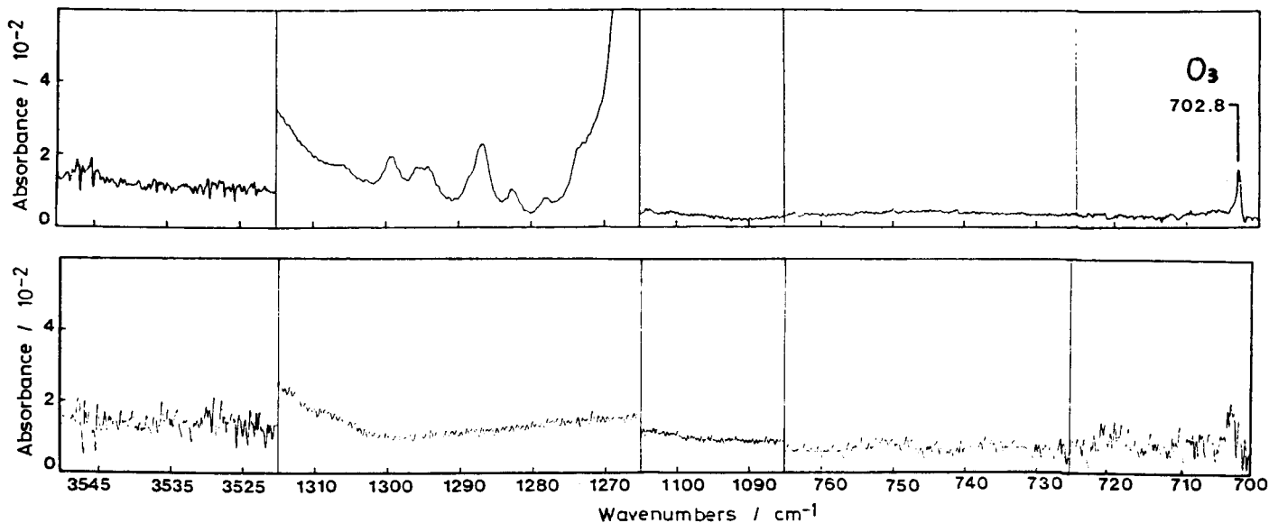
Figure 3. Infrared spectra of reaction mixtures of (a) \text{H}_2\text{O}_2/\text{O}_2 and \text{SO}_2/\text{O}_2 with the irradiation at 185 nm, and (b) \text{H}_2\text{O}/\text{O}_2 with the irradiation at 147 nm.
