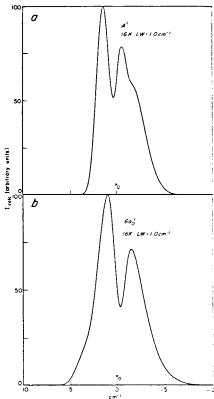
Fig. 3 - Low temperature rotational band contours of benzyl : rotational constants of Tables 1 and 2 for a ) the type A band A^1 and b ) the type B band 6a_0^1 ; LW = 1.0 \text{ cm}^{-1} and T_R = 16 \text{ K} .
