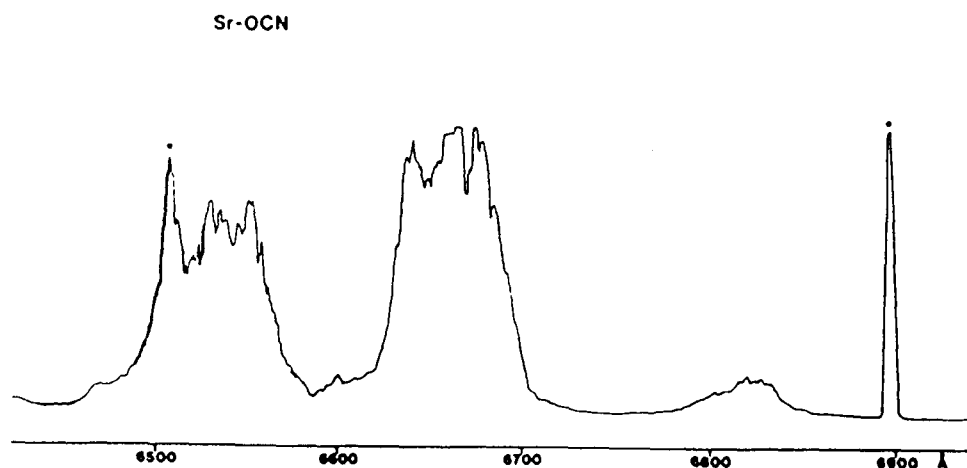
Figure 4. Laser-induced fluorescence from the \tilde{A} \leftarrow \tilde{X} transition of \text{SrOCN} . The splitting between the two strong features is due to the spin-orbit splitting in the \tilde{A}^2\Pi state. The asterisks mark the scattered light from the two exciting dye lasers on the atomic ^3P_1 \leftarrow ^1S_0 transition and the \tilde{A}_2^2\Pi_{3/2} \leftarrow \tilde{X}^2\Sigma^+ transition.
