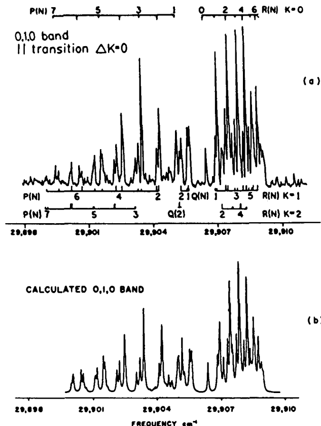
Fig. 10. (a) Spectrum of vinoxy covering approximately the same frequency region as Fig. 9, but with the rotational temperature now approximately 10^{\circ}\text{K} , (b) a simulation of spectrum in (a) based upon the molecular constants.
