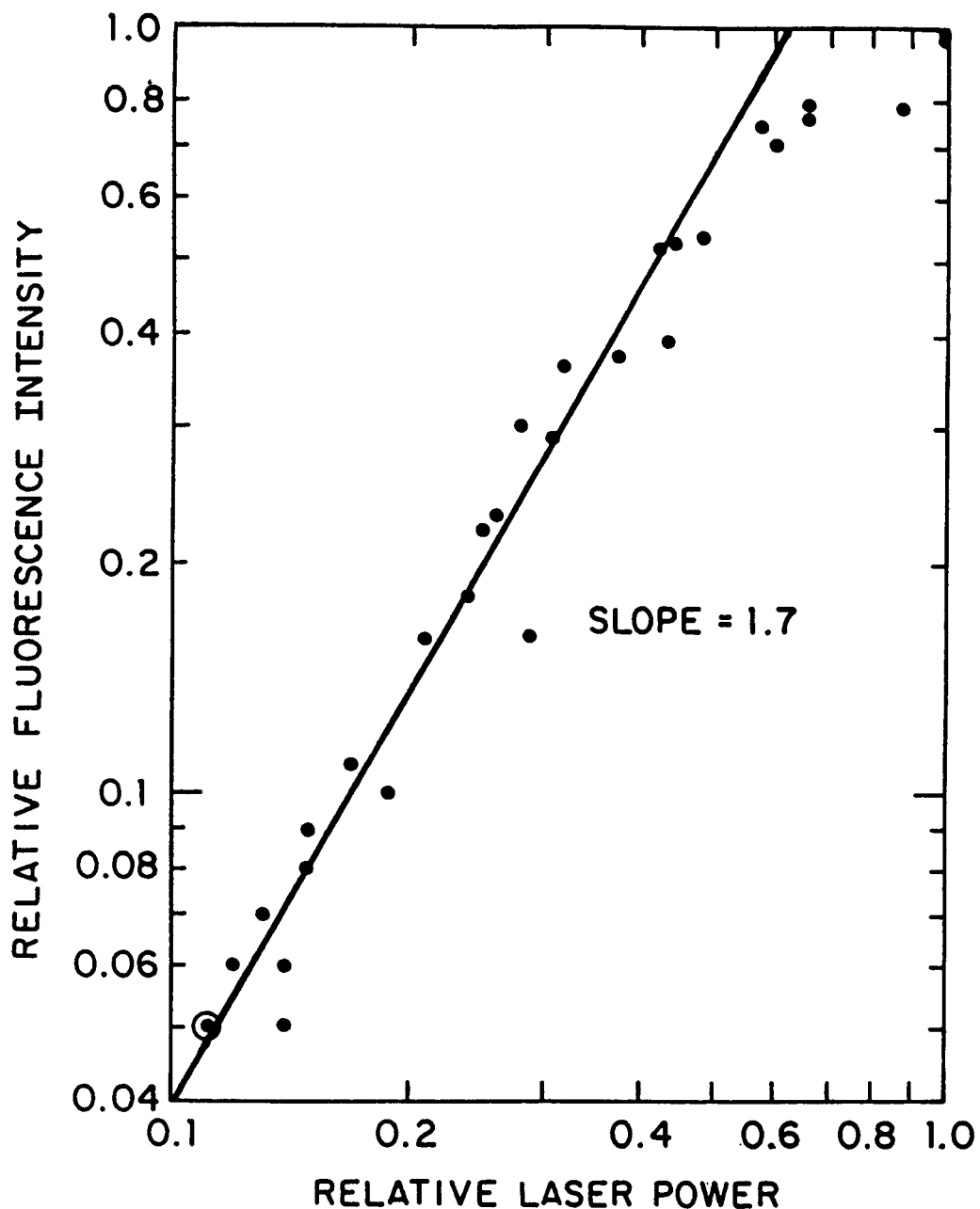
FIG. 2. POWER CURVE FOR THE PH (A→X) FLUORESCENCE.
