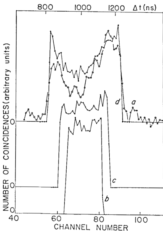
Fig. 3 - CH_4^{++} (\tilde{a}^1 E) \rightarrow CH_2^+ + H^+ + H dissociation. Experimental (curve a ) and simulated (curves b , c , d ) PIPICO spectra at E_{exc} = 42 eV. (see text for details)
