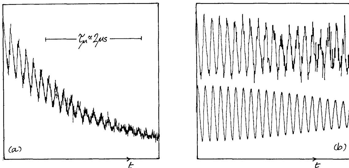
Figure 2. Positron count rate, ie number of counts as a function of muon lifetime inside the sample (a), and the extracted precession signal (b) (upper trace). The lower trace in (b) is an on-line computer fit, yielding precession frequency (here 6.5 MHz, appropriate to an applied field of 500 Gauss) and relaxation function. Notice the resemblance to Free Induction Decay signals obtained in NMR experiments following a 90^{\circ} pulse.
