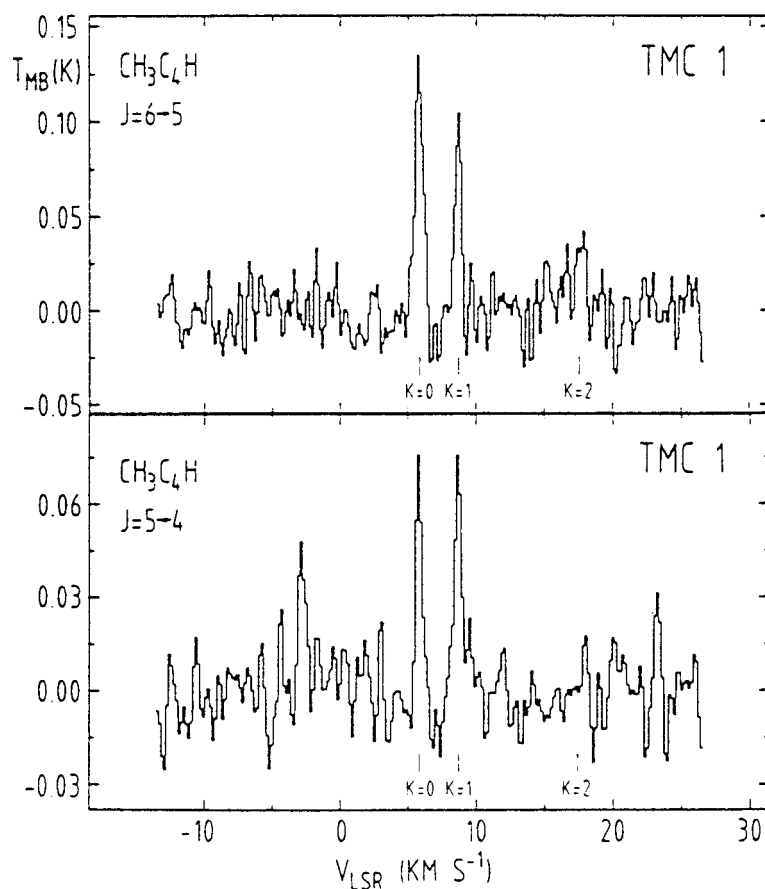
Fig. 5. - The \text{CH}_3\text{C}_4\text{H} spectrum toward TMC 1 (from Walmsley et al. 1984).
