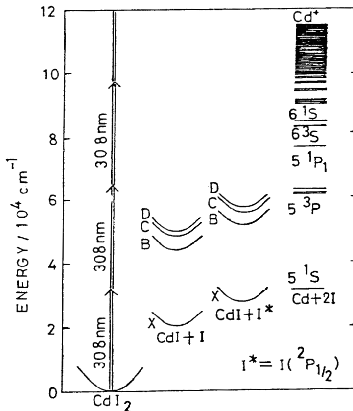
Fig. 8. Energy level diagram for CdI 2 ,
