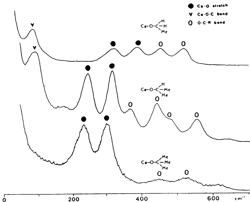
Figure 5. Laser-induced fluorescence spectra of the \text{CaOCH}_2\text{CH}_3 , \text{CaOCH}(\text{CH}_3)_2 , and \text{CaOC}(\text{CH}_3)_3 molecules (the 0-0 \tilde{A}-\tilde{X} band emission is off scale). Each vibrational feature is doubled by the spin-orbit splitting ( \sim 65 \text{ cm}^{-1} ) of the \tilde{A} state. The x-axis scale is set to zero for the \tilde{A}_1^2\Pi_{1/2} \leftarrow \tilde{X}^2\Sigma^+ 0-0 band so the scale refers to the higher frequency component of any doublet. Each pair of lines corresponds to emission from the \tilde{A} state into the vibrationally excited \tilde{X}^2\Sigma^+ state.
