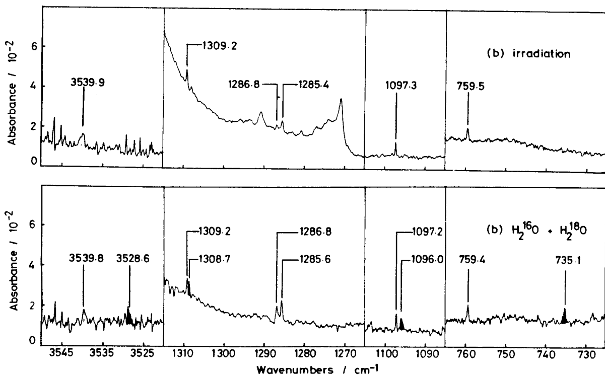
Figure 1. Infrared spectra of reactin mixtures of (a) \text{H}_2\text{O}_2/\text{Ar} and \text{SO}_2/\text{Ar} with the irradiation at 185 nm, and (b) \text{H}_2^{18}\text{O}-\text{H}_2^{16}\text{O} (1:1)/Ar and \text{SO}_2/\text{Ar} with the irradiation at 147 nm.
