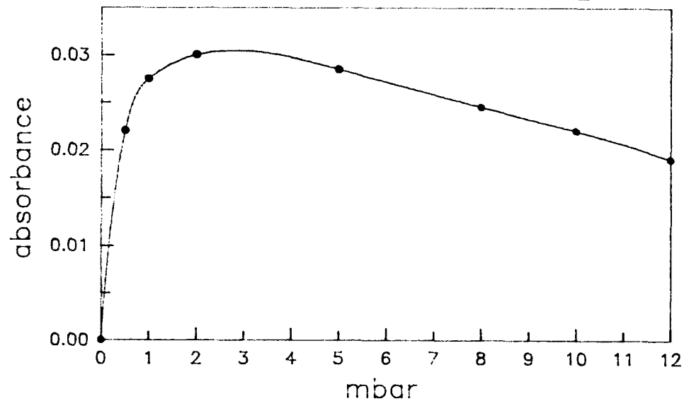
Fig.2. Yield of OH versus p(O_2)
