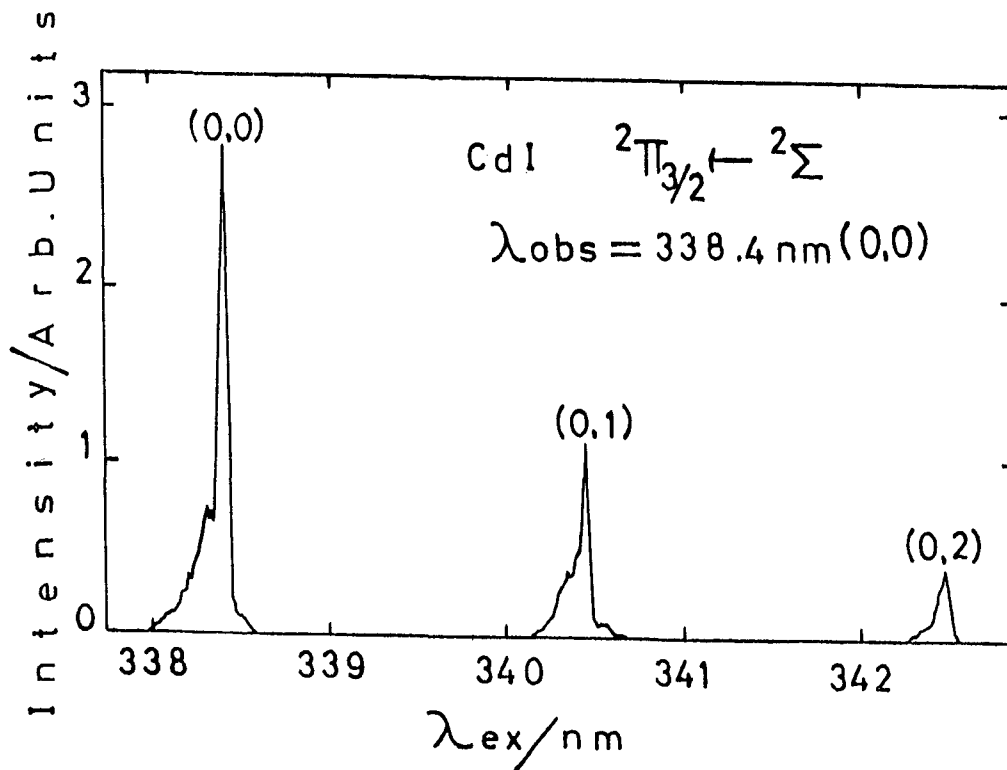
Fig. 4. LIF excitation spectra for the D \leftarrow X transition of CdI radical. \lambda_{obs} = 338.4 \text{ nm} ( D^2\Pi_{3/2} \rightarrow X^2\Sigma (0, 0) band).
