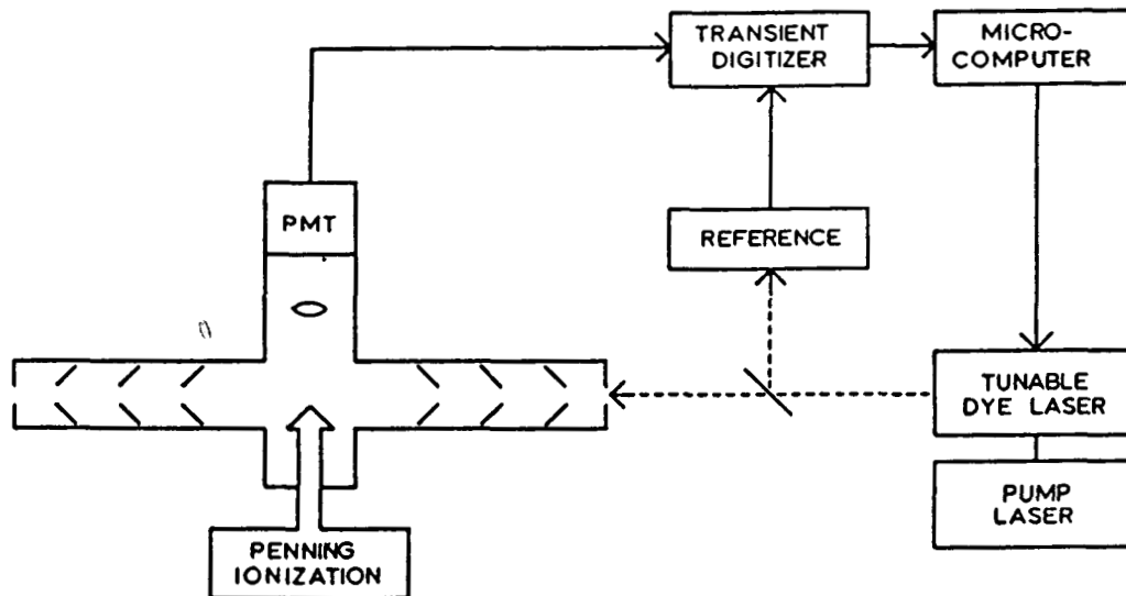
FIG.2. Schematic of the apparatus for laser-excited fluorescence spectroscopy of gas-phase cations.
