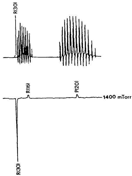
Figure 7: Post absorption and LOGE signals showing the unique situation at 1400 mTorr N_2 , where the CO_2 R(30) line has been completely absorbed.
