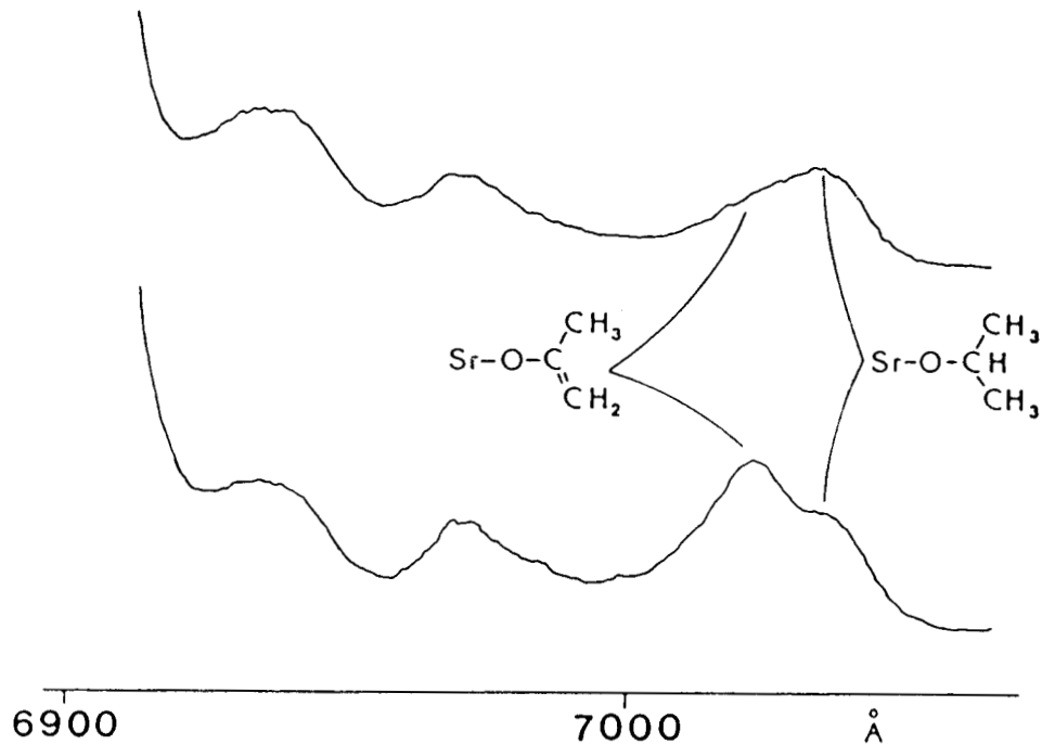
Figure 6. Laser-induced fluorescence spectra of the products of the Sr vapor plus acetone reaction. The \tilde{A}_1^2\Pi_{1/2} - \tilde{X}^2\Sigma^+ transition is off scale near 6903 Å. The upper trace corresponds to a large amount (several hundred millitorr) of acetone oxidant while the bottom trace was recorded from a flame with less than 100 millitorr of acetone. The vibrational features arise from emission from v=0 of the \tilde{A}_1^2\Pi_{1/2} state into vibrationally excited levels of the ground \tilde{X}^2\Sigma^+ state.
