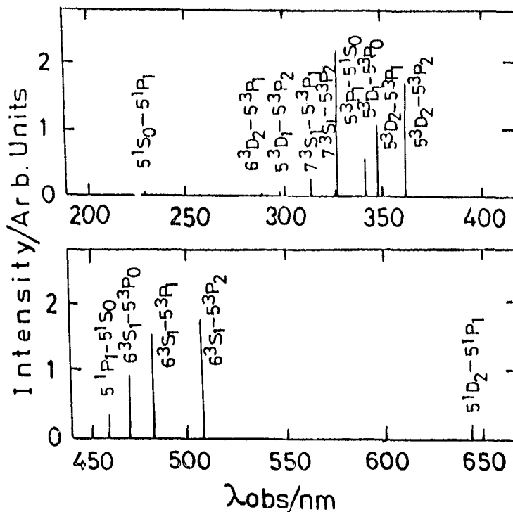
Fig. 6. Emission spectra of the cadmium atom produced by the photodissociation of CdI 2 with 308 nm XeCl laser.
