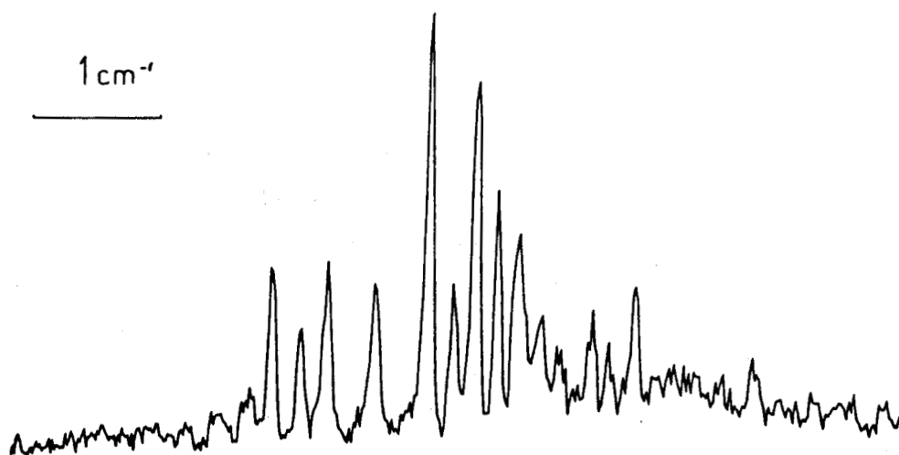
Fig. 12. Rotationally resolved spectrum of \text{C}_5\text{H}_5 . Shown is the 0-0 band of the electronic transition, \tilde{\text{A}}^2\text{A}''_2-\tilde{\text{X}}^2\text{E}''_1 .
