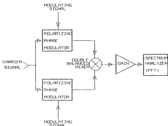
Figure 3. Block diagram of a phase bridge measurements to determine the difference in phase modulation between two phase modulators [14,15].
