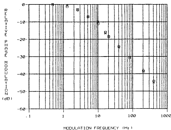
Figure 2. Relative phase modulation of the output signal as a function of the frequency of modulation. The open circles are the predictions using Eq. (7) and the half-bandwidth \nu_0/(2Q) measured from transmission experiments. The solid points are the phase modulation levels obtained from phase bridge measurements [14,15].
