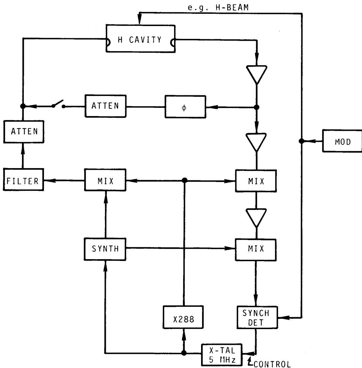
FIG. 3 Passive hydrogen concept. The crystal oscillator is locked to the hydrogen resonance using the phase sensitive dispersion lock technique. The cavity-Q is lowered using negative electronic feedback.
