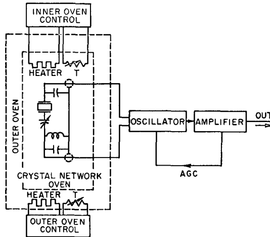
Fig. 20. Precision crystal controlled oscillator.
