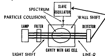
Fig. 7. Optically pumped passive gas cell
