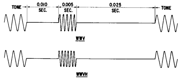
FIGURE 10.11. Characteristics of time-pulse emission from NBS radio stations WWV and WWVH.
