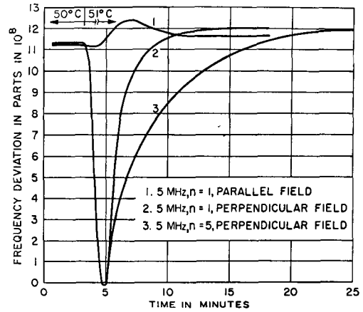
Fig. 11. Change in frequency of perpendicular and parallel field crystal vibrators due to a 1°C change in temperature.
