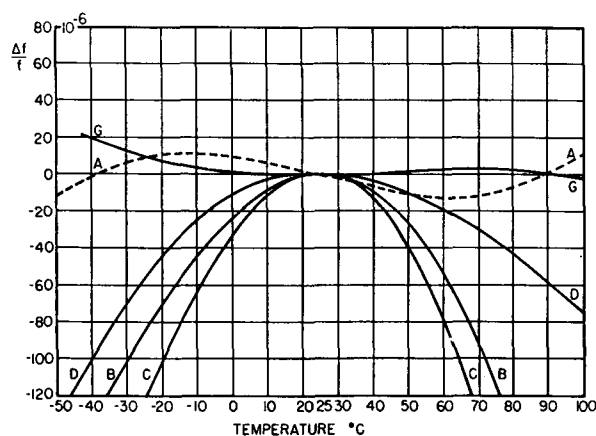
Fig. 7. Frequency-temperature characteristics of various quartz vibrators (for the explanation of letters ascribed to curves see Table I).
