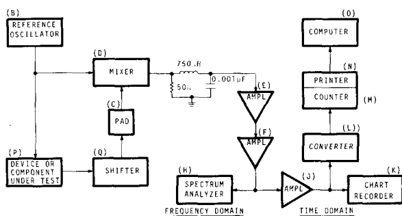
ITEMS (B) THROUGH (O) SAME AS FIGURES 8.5 AND 8.11 (P) ANY DEVICE OR COMPONENT UPON WHICH NOISE MEASUREMENTS ARE DESIRED (AMPLIFIERS, FILTERS, CAPACITORS, CABLES, PADS, ETC.) (Q) NBS ADJUSTABLE PHASE SHIFTER, 5MHz (SEE FIGURE 8.15)
