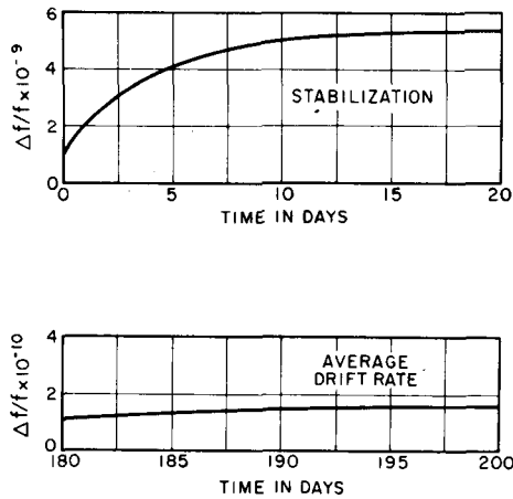
Fig. 21. Initial stabilization period and drift rate of 2.5-MHz precision oscillators.
