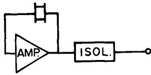
Fig. 14. General purpose crystal controlled oscillator.
