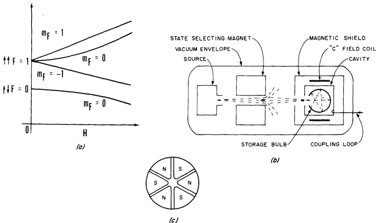
Fig. 3.6. Part (a) gives the energy levels for the ground electronic state ( 1^2S_{1/2} ) of the H atom. Part (b) is a schematic of the H maser. Part (c) is the end view of the hexapolar state selecting magnet typically used in an H maser.
