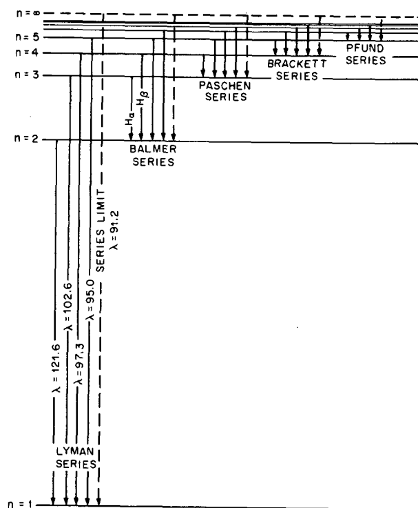
Fig. 3.1. The energy level diagram of the hydrogen atom as obtained from the Bohr theory. The wavelengths (of the Lyman Series) are given in nanometers, nm (1000 Angstroms equals 100 nm).
