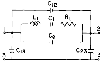
Fig. 1. Equivalent circuit of a quartz crystal unit.
