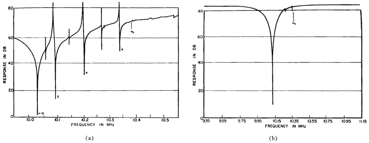
Fig. 5. Reduction in unwanted responses in a crystal vibrator by "trapped energy" principle. In (a), the response n=0 is the main mode; the other responses are inharmonic overtones; \omega_c is the cutoff frequency.
