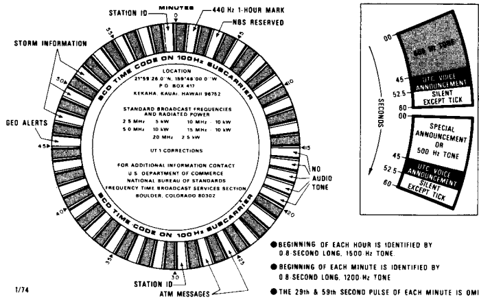
FIGURE 10.10. Hourly broadcast format of WWV (a) and WWVH (b).
