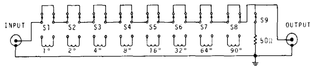
RG174/U CABLE WAS USED FOR EACH SEGMENT OF PHASE SHIFT CALCULATED AT \sim 10 cm PER DEGREE AT 5 MHz.
