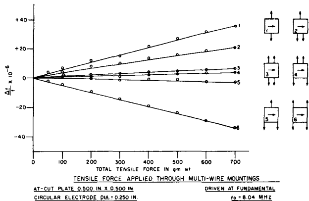
Fig. 12. Change in frequency of A-type vibrators due to external forces. The squares represent the crystal plates; the arrows in the squares indicate the direction of the X-axis, and the arrows outside indicate the applied tensile forces.
