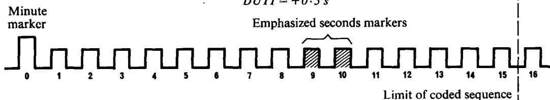
FIGURE 4 DUT1 = -0.2 s
