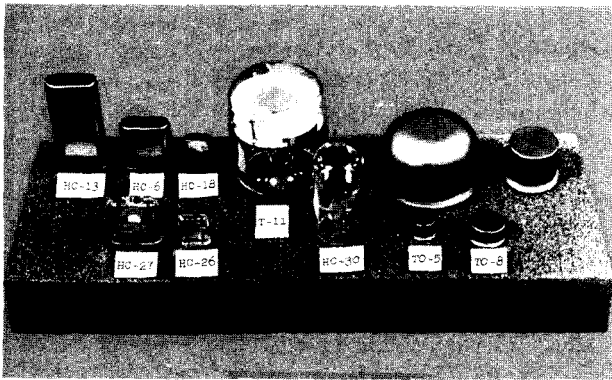
Fig. 3. Quartz crystal unit holders.
