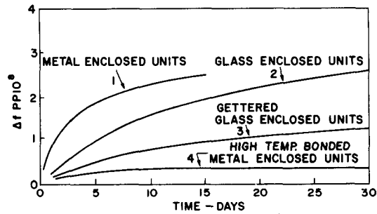
Fig. 9. Aging of metal and glass enclosed 5-MHz crystal units.
