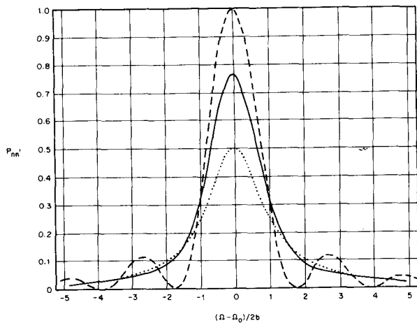
Fig. 3.2. Theoretical curves of P_{nm} . The dashed curve is obtained from eq (3.4) by setting \tau = \pi/(2b) . The full curve is obtained from an average over the velocity distribution and with an optimum \tau ( \tau = 1.2\pi/(2b) ). The dotted curve comes from an average over the same velocity distribution but with \tau \gg \pi/(2b) . (See text for further details.) (This figure is a modification of Fig. V.1 of Molecular Beams by Norman F. Ramsey, copyright by Oxford University Press, 1956).
