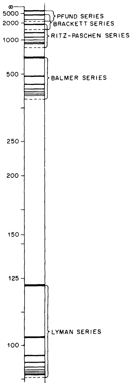
Fig. 3.3. Schematic diagram of the emission spectrum of the hydrogen atom. The intensity of the emission is roughly indicated by the thickness of the lines. The dotted lines are series limits. The wavelength scale is in nanometers. (This figure is a modification of Fig. 8 of Atomic Spectra and Atomic Structure by Gerhard Herzberg, copyright by Dover Publications, 1944.)
