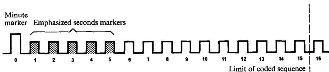
FIGURE 3 DUT1 = +0.5 s
