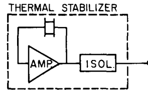
Fig. 19. Oscillator for severe mechanical and temperature environments.
