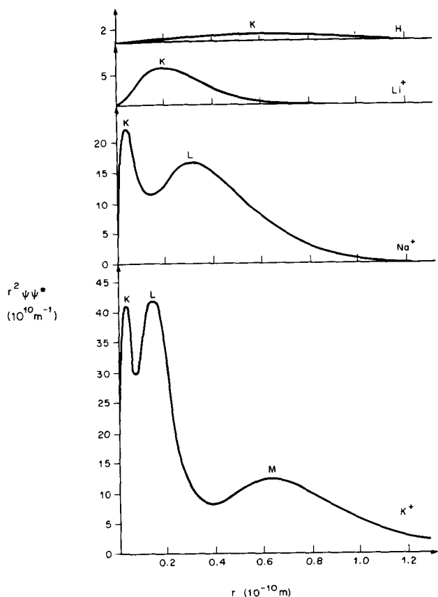
Fig. 3.4. Charge distribution for the ground states of H, Li + , Na + , and K + . The concentrations of charge (corresponding to the maxima) in these distributions are analogous to the orbits of the Bohr theory and are called shells. The area under the curves is proportional to the number of electrons in the atom. The vertical axis is equal to r^2\psi\psi^* where r is in meters. (This figure is a modification of Fig. 54 of Atomic Spectra and Atomic Structure by Gerhard Herzberg, copyright by Dover Publications, 1944.)
