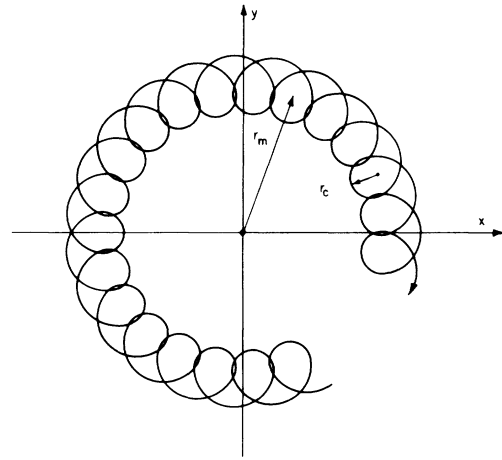
FIG. 1. Orbit of an ion in a Penning trap, projected onto the xy plane. The magnetic field direction is out of the drawing and the charge of the ion is assumed to be positive.
