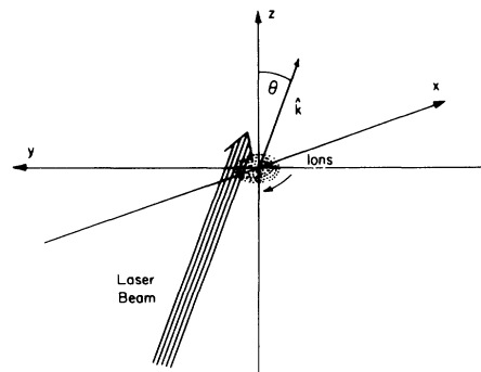
FIG. 3. Nonuniform laser beam configuration which is capable of cooling all three modes of motion of an ion in a Penning trap. The trap coordinate axes are indicated. The ion cloud is at the origin, and the direction of the magnetron rotation is indicated by an arrow. The laser light propagates in the \hat{k} direction, which lies in the xz plane. The laser beam is focused so that it is more intense for y > 0 than for y < 0 .
