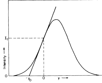
FIG. 2. Intensity profile of nonuniform laser beam. I_1 is the intensity at y=0 and I_1/y_0 is its slope. The tangent to the curve is used as an approximation to the actual profile in the calculation.
