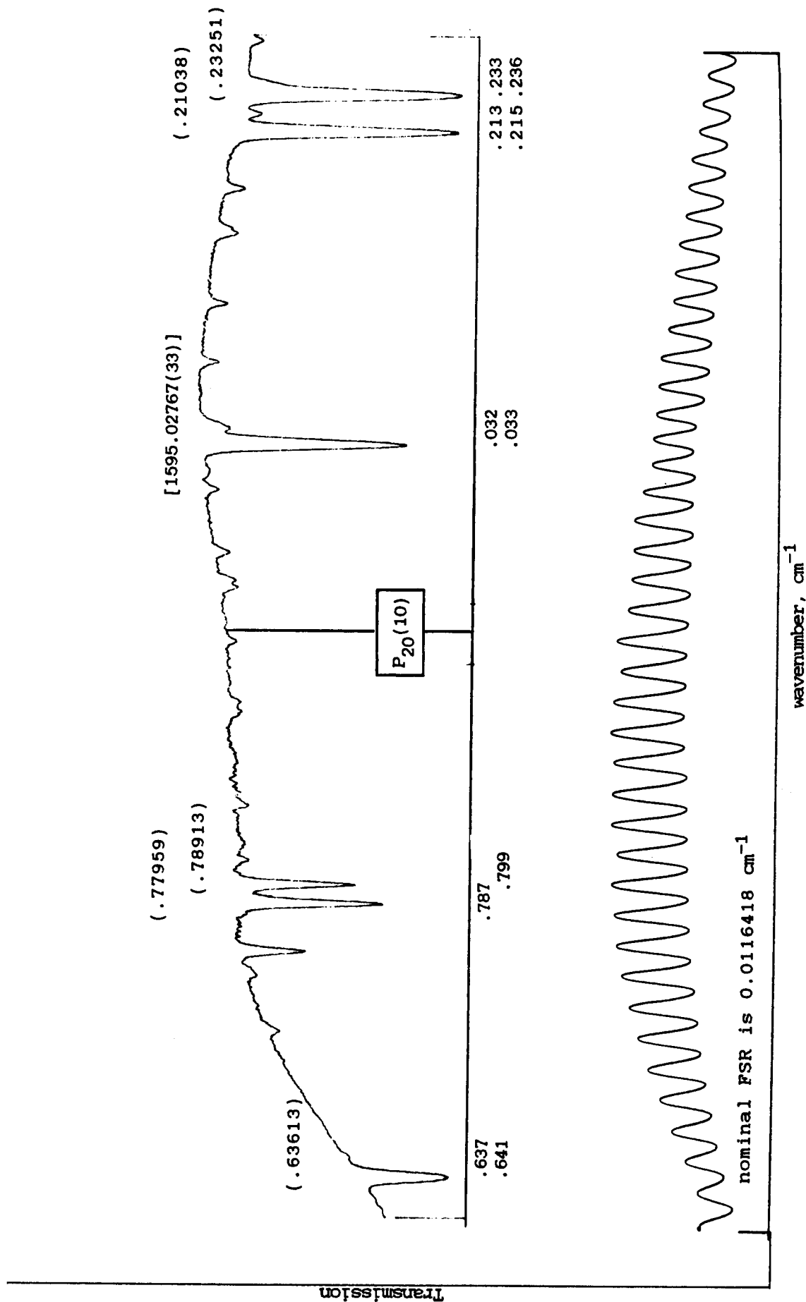
Fig. A-3. Nitrogen dioxide spectra in the vicinity of the P 20 (10) CO laser line at 1594.91939 cm -1 .
