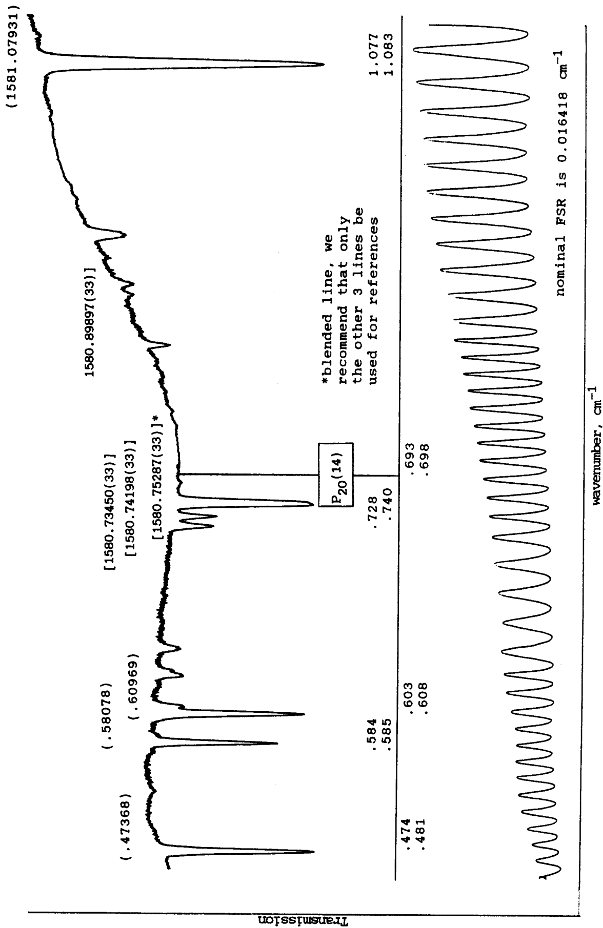
Fig. A-1. Nitrogen dioxide spectra in the vicinity of the P 20 (14) CO laser line at 1580.77335 cm -1 .
