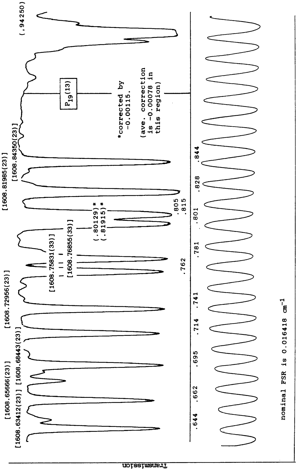
Fig. A-5. Nitrogen dioxide spectra in the vicinity of the P 19 (13) CO laser line at 1608.89765 \text{cm}^{-1} .
