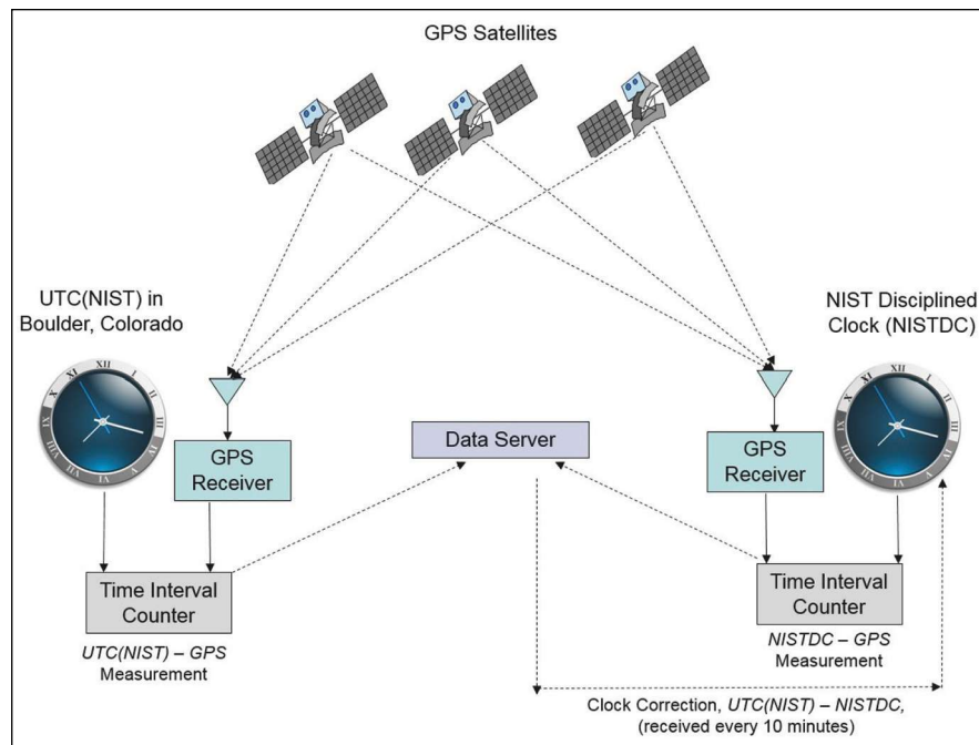
FIGURE 4 NIST disciplined clock system utilizing the common-view GPS method.
