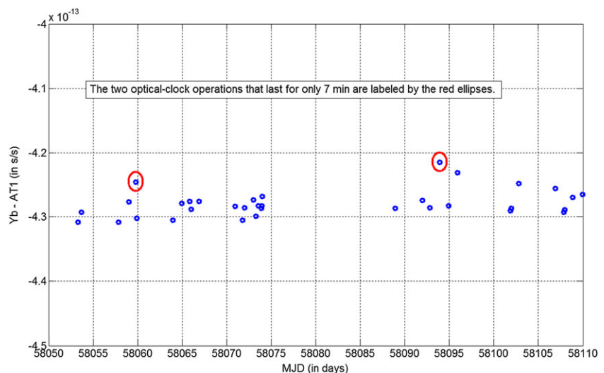
FIGURE 9 Average of “Yb – AT1” for the ongoing campaign [Color figure can be viewed at wileyonlinelibrary.com and www.ion.org ]
