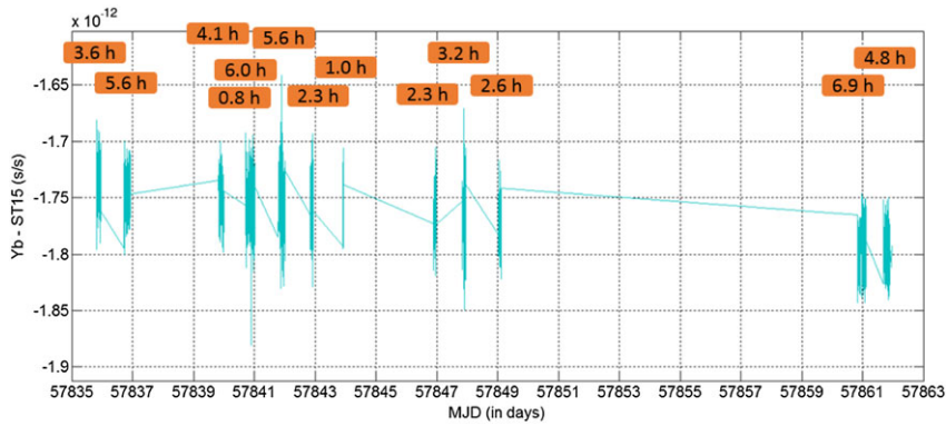
FIGURE 6 Comparison of the Yb optical clock and a NIST hydrogen maser (ie, ST15) for the initial campaign [Color figure can be viewed at wileyonlinelibrary.com and www.ion.org]
