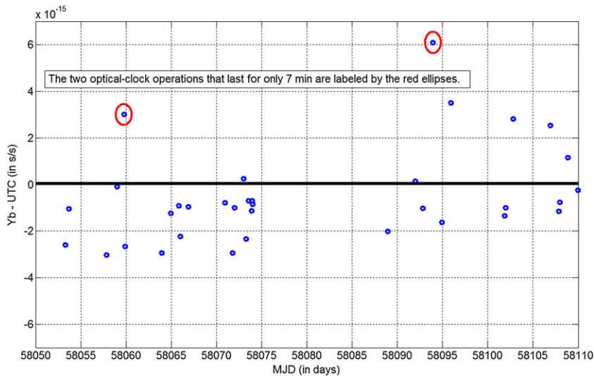
FIGURE 10 Average of “Yb – UTC,” for the ongoing campaign [Color figure can be viewed at wileyonlinelibrary.com and www.ion.org ]
