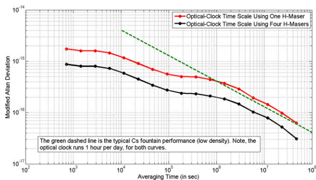
FIGURE 5 The simulated results of steering an ensemble of masers to an optical frequency reference that runs 1 hour per day. An ensemble of four masers steered to an optical clock running 1 hour per day is more stable than a cesium fountain for all averaging times [Color figure can be viewed at wileyonlinelibrary.com and www.ion.org ]
