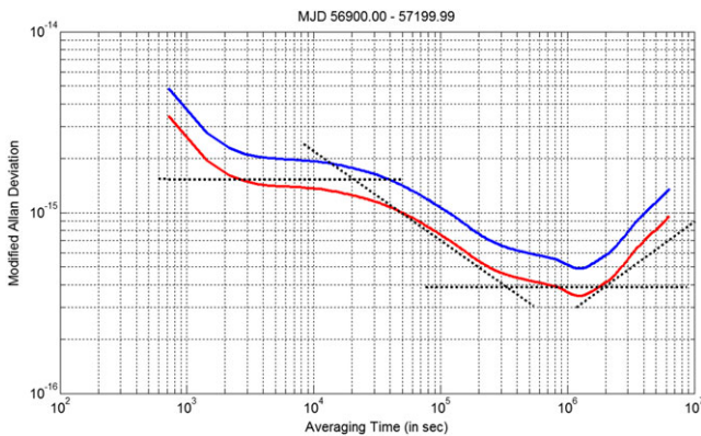
FIGURE 1 The blue curve shows the frequency stability of the time difference between two NIST H-masers. The red curve shows the estimated frequency stability of a single H-maser, assuming that the two masers have the same statistical characteristics. We model the stability as shown by the black dotted lines [Color figure can be viewed at wileyonlinelibrary.com and www.ion.org ]
