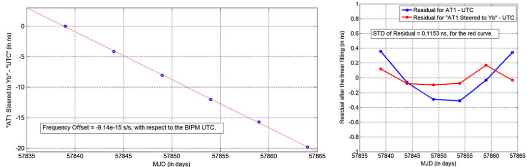
FIGURE 8 Steered AT1 versus UTC (left) and the residual after the linear fitting (red curve in the right plot) for the initial campaign [Color figure can be viewed at wileyonlinelibrary.com and www.ion.org]
