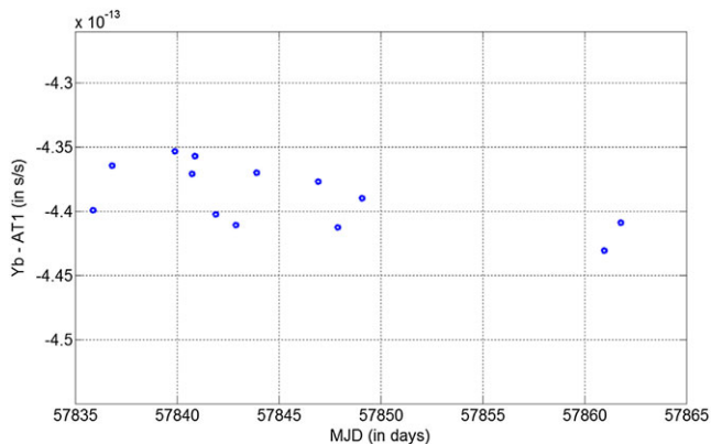
FIGURE 7 Average of “Yb – AT1” for the initial campaign [Color figure can be viewed at wileyonlinelibrary.com and www.ion.org]
