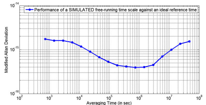
FIGURE 2 Frequency stability of a simulated free-running time scale with one maser against an ideal reference time [Color figure can be viewed at wileyonlinelibrary.com and www.ion.org ]
