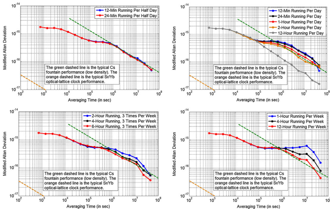
FIGURE 4 Performance of a time scale steered to an intermittently operating optical clock. A variety of running schedules are studied in this figure [Color figure can be viewed at wileyonlinelibrary.com and www.ion.org ]
