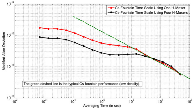
FIGURE 3 Performance of a time scale steered to a continuously operating cesium fountain. The green dashed line shows the performance of the cesium fountain. The solid curves show the stability of a steered time scale that contains either one or four masers [Color figure can be viewed at wileyonlinelibrary.com and www.ion.org ]
