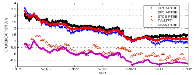
violet : PPP Lab( k )-PTB; Triangle : TWSTFT Lab( k )-PTB; Red : PPP \text{Std}_B -PTBB ( \text{Std}_B is mean of BP0U/blue and BP1C/black)
