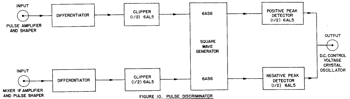
FIGURE 10. PULSE DISCRIMINATOR
