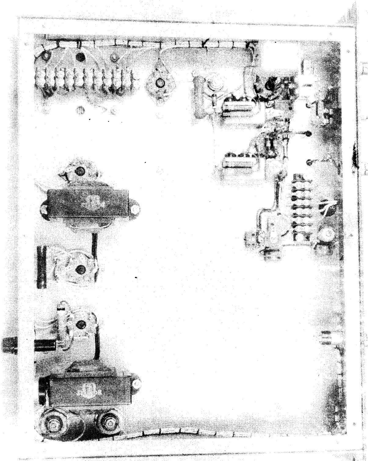
Fig. 35. ADJUSTABLE FREQUENCY OSCILLATOR; 500 TO 600 KC/S (BOTTOM VIEW).
