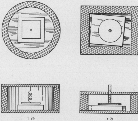
Fig. 1—Types of simple quartz plate holder.
