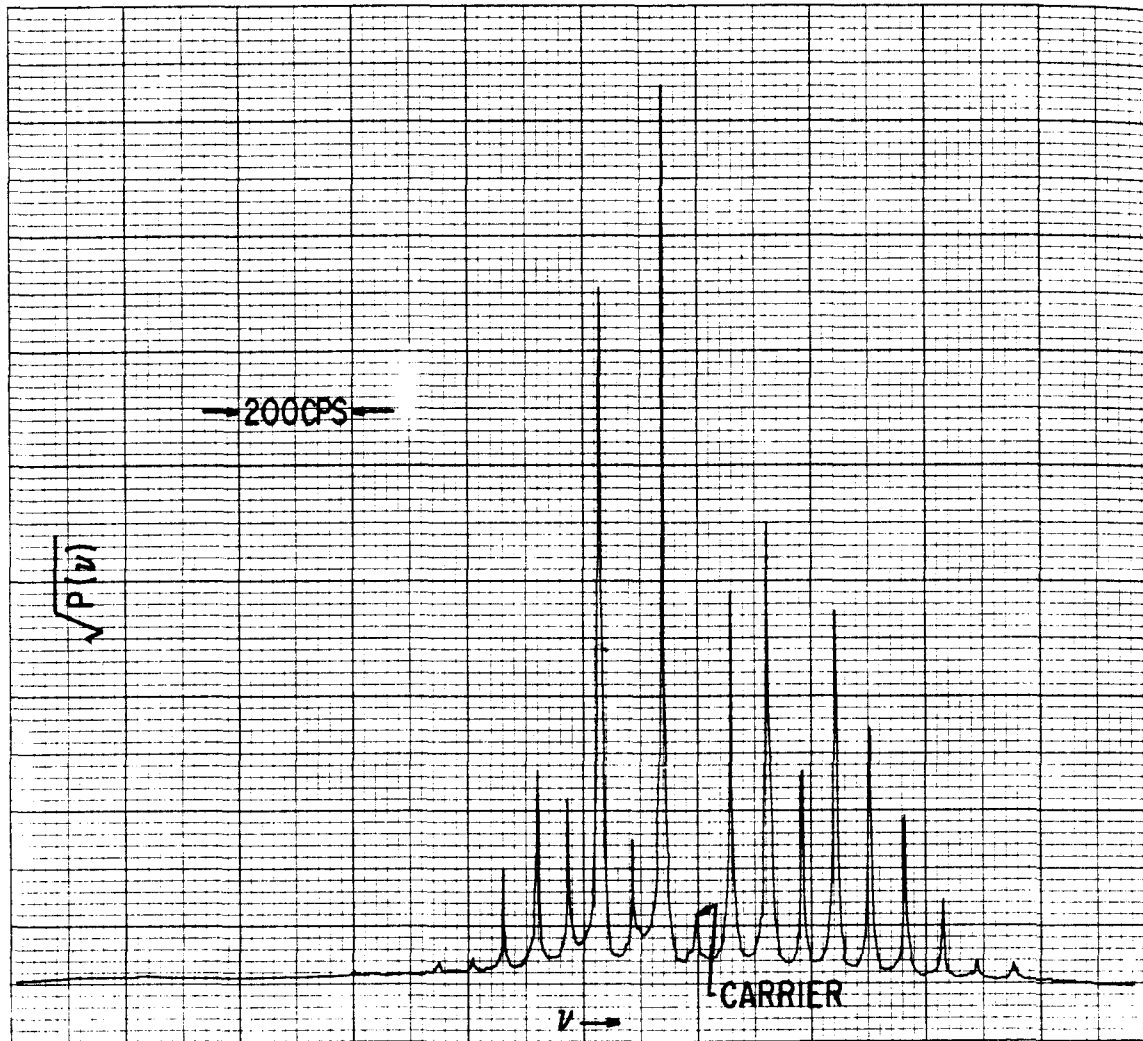
Fig. 4 This spectrum was obtained from the same oscillator as Figure 3. At the time this trace was made, however, the oscillator was equipped with 60 cps, ac filaments. (Note the different frequency scale).
