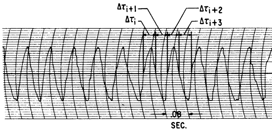
Fig. 8 Recording of direct beat note between free running oscillator and maser. A numerical analysis of these recordings could also be run to determine the power spectrum.
