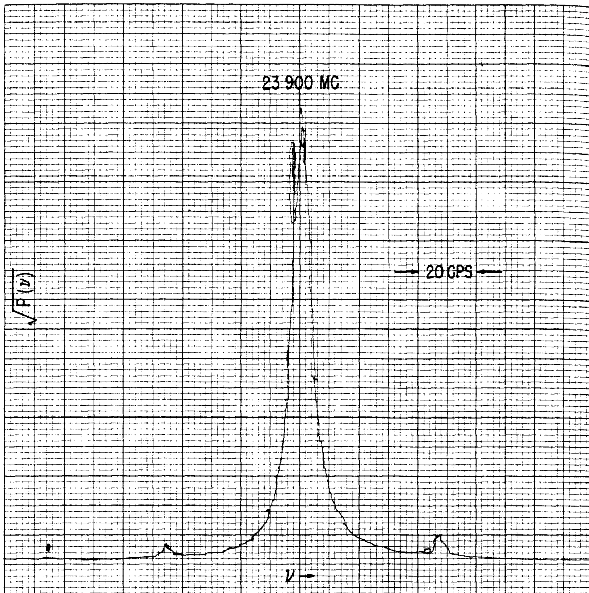
Fig. 6 This spectrum was obtained by intentionally frequency modulating the oscillator of Fig. 5 at a 50 cps rate. The total swing in frequency of the oscillator was about 2 parts in 10^{10} peak to peak, (note the small sidebands at 50 cps on either side of the central peak).
