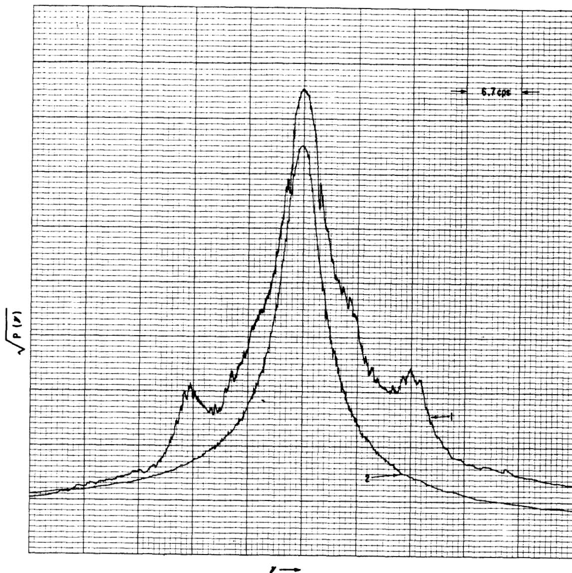
Fig. 3 Trace 1 is a high resolution spectrum of the central peak of a 10 Mc quartz crystal oscillator whose crystal was thermostated in a liquid helium cryostat [5] . The oscillator was equipped with DC filaments but still exhibited 60 cps sidebands about 30 db below the central peak (not shown in this figure). This oscillator operates at about 13.4 cps above 10 Mc and apparently some pickup of the standard is responsible for the sidebands shown in this trace. Trace 2 is the response curve of the spectrum analyser.
