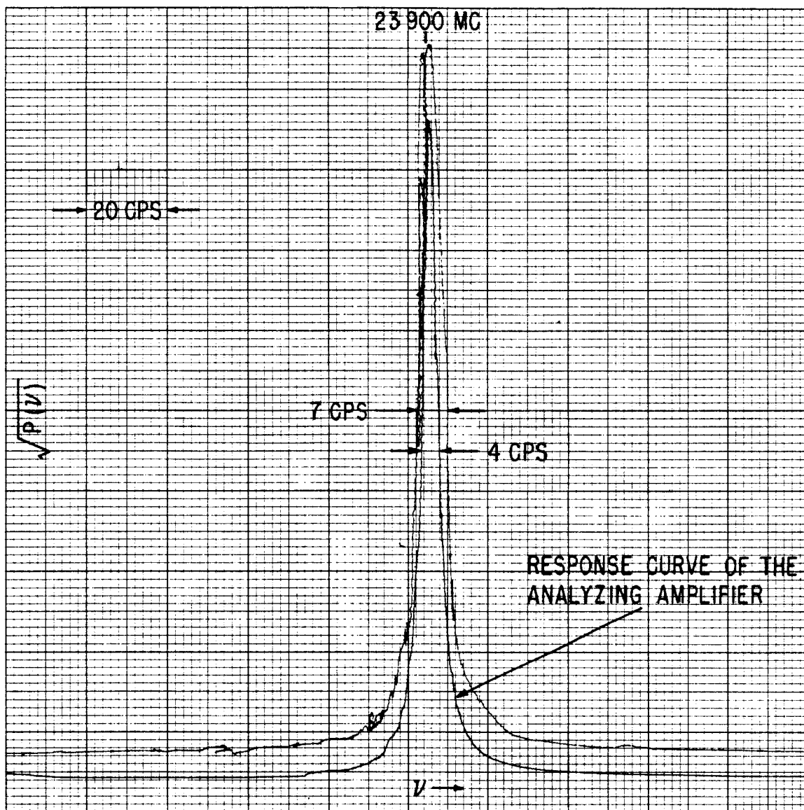
Fig. 5 This spectrum was obtained by analysing the direct beat note between the free running oscillator-multiplier-chain-system and the ammonia maser. It is this oscillator which is phase locked to the maser to give a relatively pure signal to be used in the analysing of other oscillators. The response curve of the analyser was obtained by replacing the maser-oscillator beat note by the signal from a high quality signal generator.
