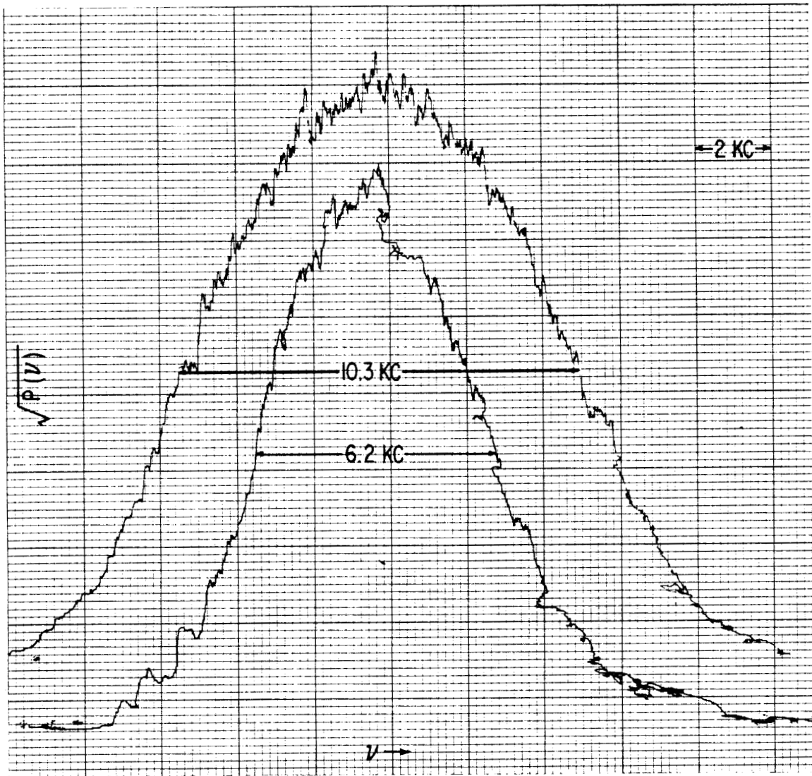
Fig. 7 This is a spectrum of a 100 kc oscillator, again multiplied 145,800 in frequency, located two floors above the room containing the maser-spectrum-analyser system. The signal apparently picked up noise in the long cables connecting the two rooms. The upper trace was taken approximately one hour after the multiplier chain in the spectrum analyser was first turned on, and the lower trace about 6 hours after the chain was turned on, showing the effect of warm up time of a multiplier chain on a noisy signal. (Note the scale).
