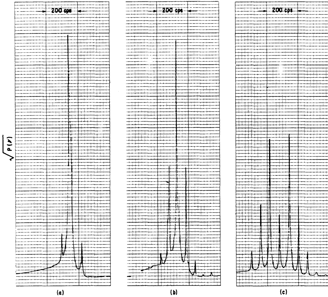
Fig. 2 Figure 2(a) shows the square root of the power spectrum for a 3.3 Mc signal. Figures 2(b) and 2(c) show the same signal after being multiplied in frequency by factors of 3 and 9 respectively.
