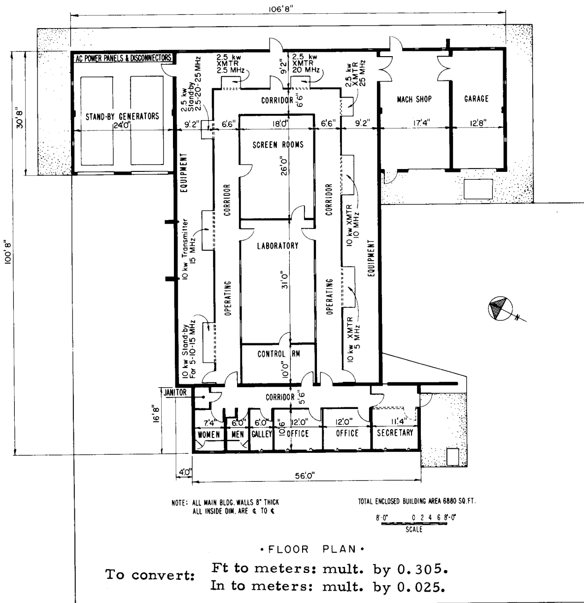
Figure 5. Floor plan of the WWV transmitter building.
