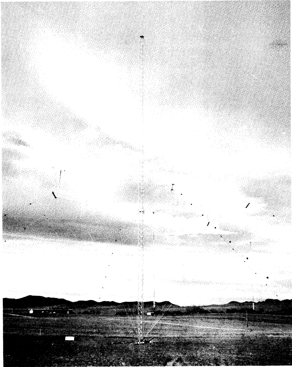
Figure 13. A view of one of the 2.5 - 25 MHz standby antennas.
