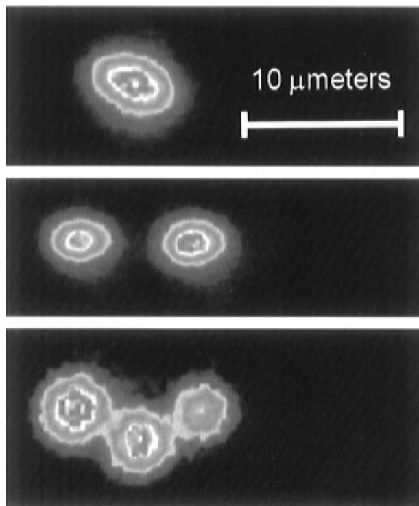
Figure 1. Image of one, two, and three beryllium ( {}^9\text{Be}^+ ) ions held in a rf (Paul) electromagnetic trap. The ions are illuminated by resonant laser light, and the scattered fluorescence is collected. The resolution (a few micrometers) is limited by the optical imaging system and is much larger than the actual size of the atomic wavepackets (a few nanometers). All of the experiments reported here deal with a single trapped ion.
