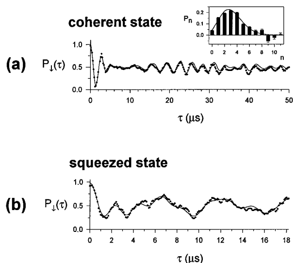
Figure 4. (a) P_{\downarrow}(\tau) for a coherent state driven with a Raman probe tuned to the blue sideband (Stokes transition), showing collapse and revival behavior. The solid curve is a single-parameter fit to a coherent state distribution, yielding \langle n \rangle = 3.1(1) . The inset shows the results of inverting the time-domain data by employing a Fourier cosine transform at the known Rabi frequencies \Omega_{n,n+1} , fitted to a Poissonian distribution, yielding \langle n \rangle = 2.9(1) . (b) P_{\downarrow}(\tau) for a squeezed state driven by the blue sideband interaction, showing a complicated behavior involving many vibrational levels. The solid curve is a single-parameter fit to a squeezed state distribution, yielding a squeeze parameter \beta = 40(10) . Each data point in both traces represents an average of \sim 4000 measurements, or 1 s of integration.
