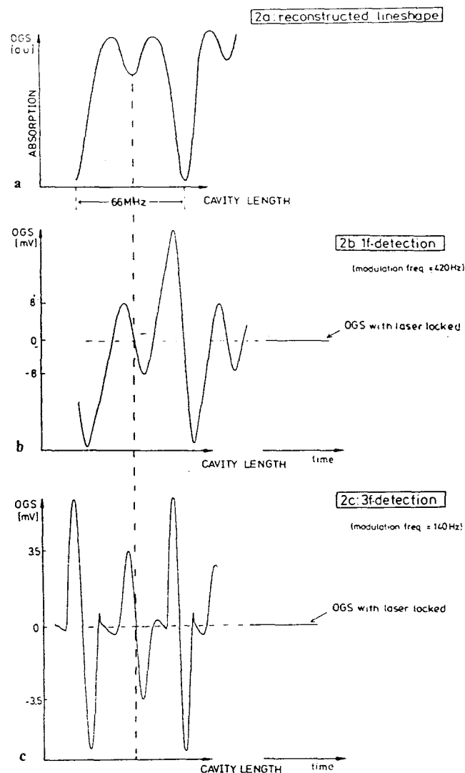
Fig. 2a-c. Optogalvanic signals (OGS) at 1.3 Torr as a function of resonator length. (a) Reconstructed non-"derivative" lineshape, (b) 1f detection: lock-in time constant 50 ms, (c) 3f detection: lock-in time constant 50 ms
