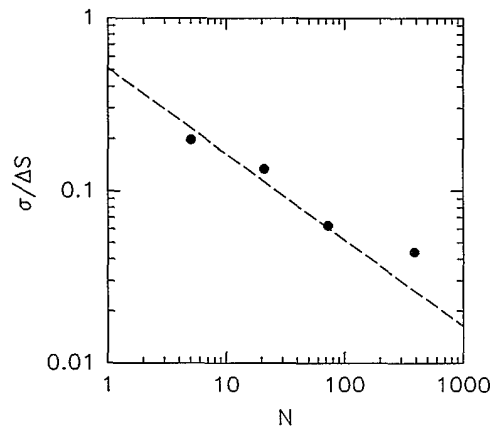
FIG. 12. Plot of the normalized standard deviations as a function of N , the number of ^9\text{Be}^+ ions. The quantity \sigma/\Delta S is the ratio of the experimental standard deviation on the sides of the resonance to the difference in the signal between the peaks and the dip. The dashed line is the theoretical prediction for the contribution from quantum projection noise alone.
