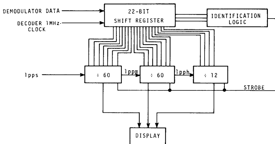
Fig. 11. Block diagram of a digital clock that may be interconnected to active TV line-1 demodulator.
