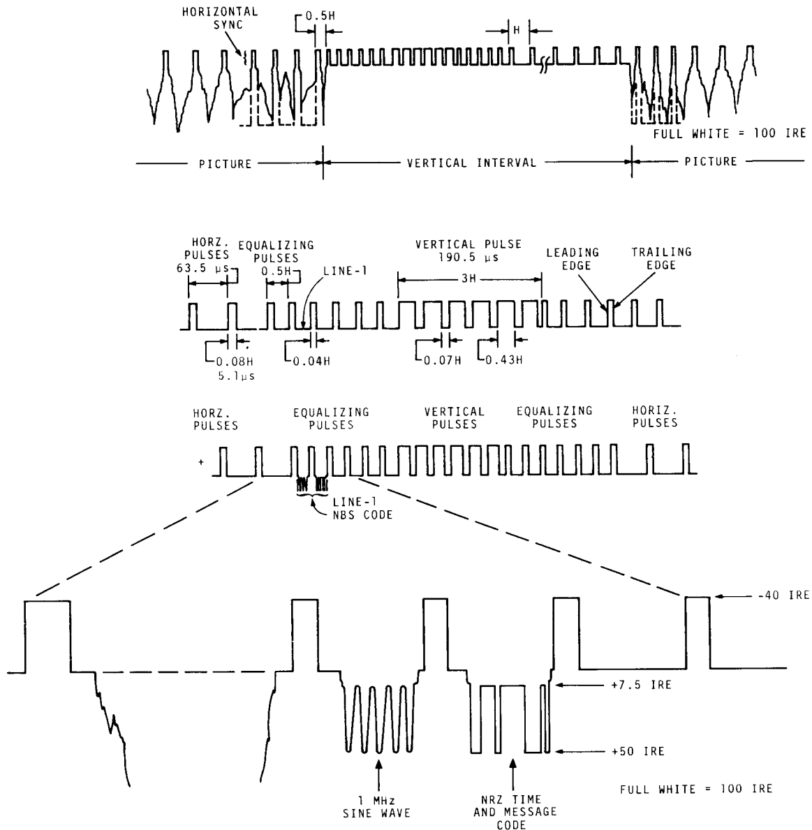
Fig. 1. Waveforms of U.S. television format, vertical interval, and NBS experimental line-1 code ( H = horizontal line period of 1/15\ 750 s or 63.5\ \mu\text{s} ).
