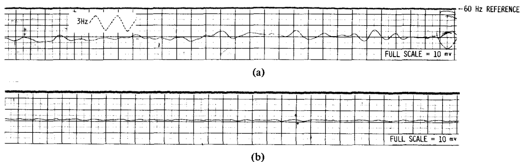
Fig. 6. 1-MHz oscillator loop error voltage when (a) locked to signal from New York as received in Boulder (note dominant 3-Hz noise) and (b) locked to local time code generator. Measurements taken at NBS Boulder receiver site.
