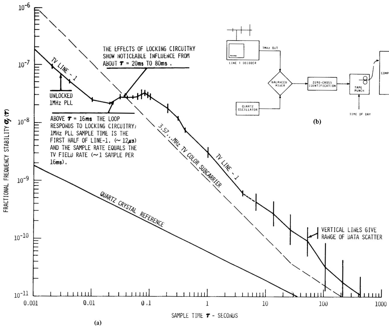
Fig. 7. (a) \sigma_{f_{req}} versus \tau of active TV line 1, 1-MHz PLL. ( 1 \text{ ms} < \tau < 15 \text{ min} ). The same measure of 3.57954... MHz PLL derived from network color subcarrier is shown for comparison (dashed line). (b) Schematic for measuring time domain stability for 6 \text{ s} < \tau < 400 \text{ s} .
