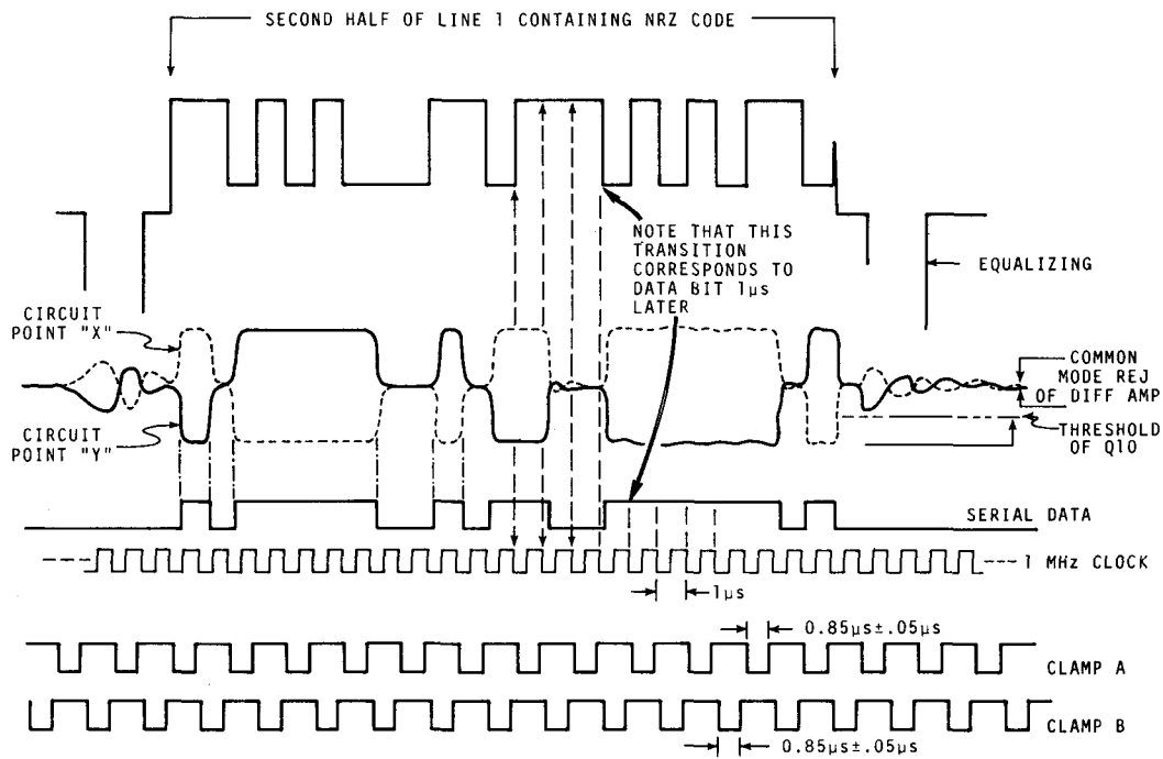
Fig. 10. Waveform diagram indicating the action of demodulator on typical NRZ code.
