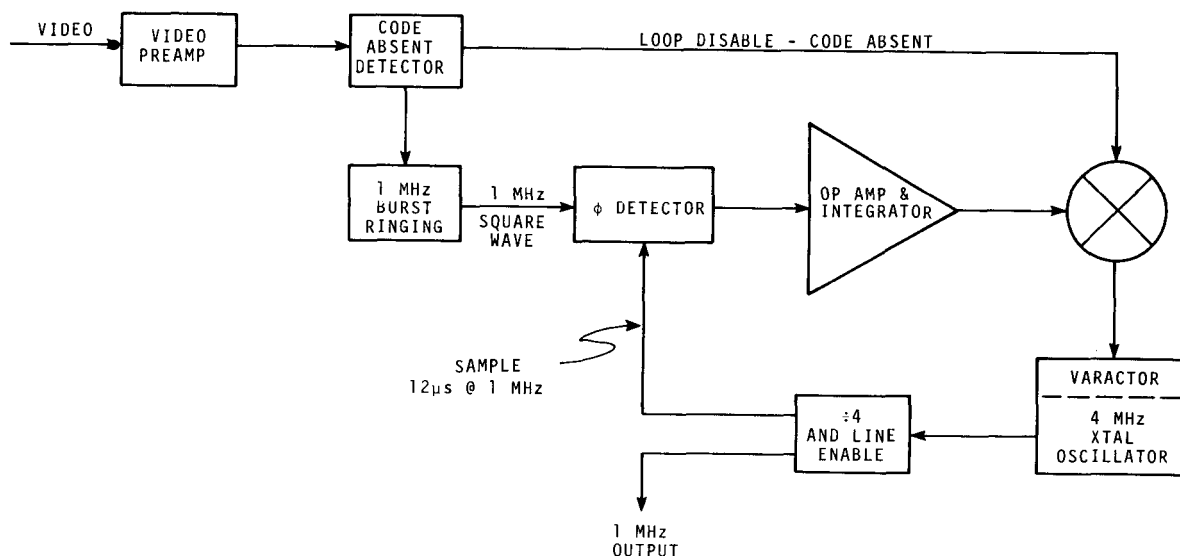
Fig. 5. Block diagram of phase-locked oscillator that uses TV line 1, 1-MHz sine wave as reference.
