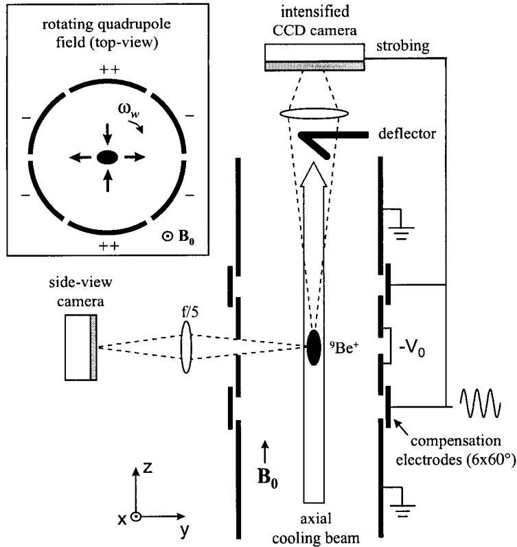
FIGURE 1. Schematic view of the cylindrical trap with real space imaging optics for the side-view camera and Bragg diffraction detection system for the axial cooling beam. Cross section of the rotating quadrupole field (in the x - y plane) is shown in the insert. From Ref. [20].
