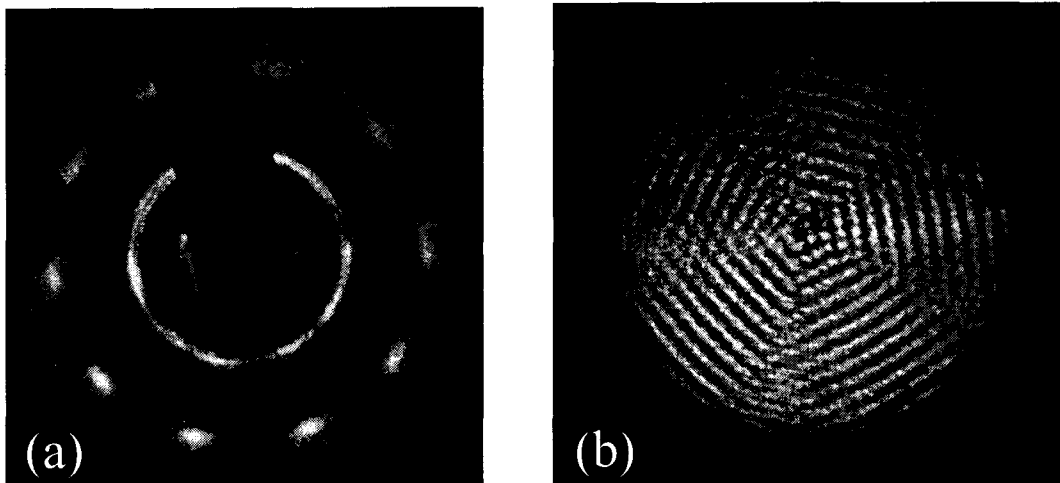
FIGURE 6. Five-fold Bragg scattering and real-space patterns obtained by strobing the intensified CCD camera synchronously with the rotating electric field perturbation. (a) Bragg scattering pattern obtained on an N \sim 1.2 \times 10^5 ion plasma phase-locked with a rotating dipole field at \omega_r = 2\pi \times 166.84 kHz. Here V_o = 500 V and \alpha = 2.6 . (b) Real-space image of a disk-like plasma consisting of 4 horizontal planes in the plasma center. The rotating dipole field was used to set \omega_r = 2\pi \times 74.35 kHz.
