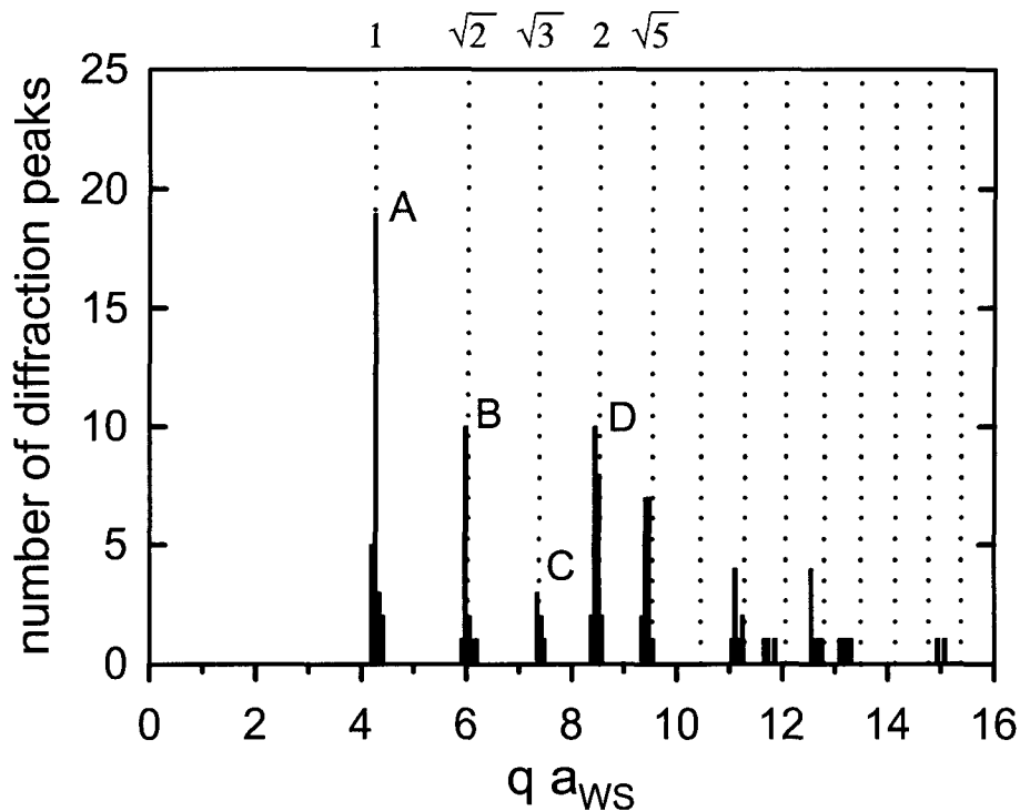
FIGURE 3. Histogram showing the numbers of peaks (not intensities) observed as a function of q a_{WS} (defined in the text) for 30 time-averaged Bragg scattering patterns obtained on two different spherical plasmas with N > 2 \times 10^5 . The dotted lines show the expected peak positions for a bcc crystal, normalized to the center of gravity of the peak at A (corresponding to Bragg reflections off \{110\} planes). From Ref. [18].
