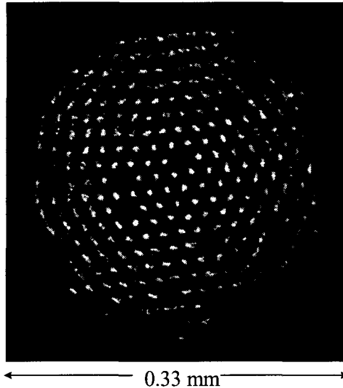
FIGURE 5. Strobed top-view image of a small N \sim 300 {}^9\text{Be}^+ ion plasma phase-locked with a rotating dipole field at \omega_r = 2\pi \times 65.7 kHz. Heavier-mass ions are located outside the {}^9\text{Be}^+ ions.
